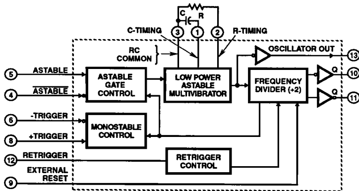
FIGURE 1. CD4047BMS LOGIC BLOCK DIAGRAM
