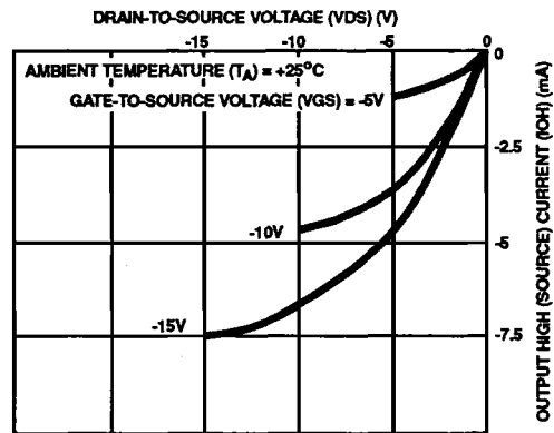
FIGURE 7. MINIMUM OUTPUT HIGH (SOURCE) CURRENT CHARACTERISTICS
