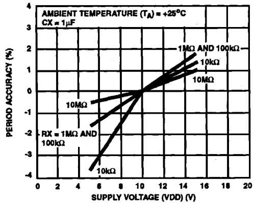
FIGURE 11. TYP. ASTABLE OSCILLATOR Q, \bar{Q} PERIOD ACCURACY vs SUPPLY VOLTAGE
