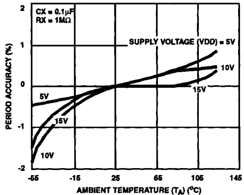
FIGURE 15. TYP. ASTABLE OSCILLATOR Q, \bar{Q} PERIOD ACCURACY vs AMBIENT TEMPERATURE (LOW FREQ.)
