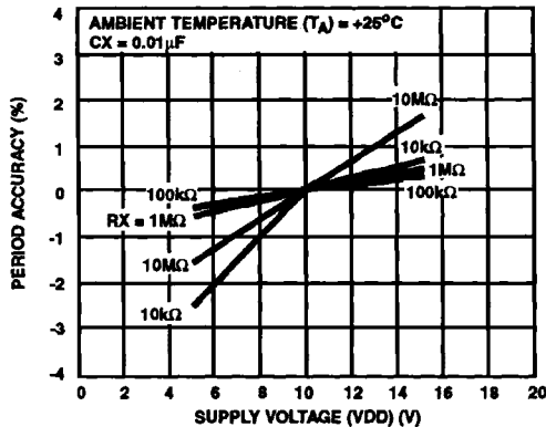
FIGURE 12. TYP. ASTABLE OSCILLATOR Q, \bar{Q} PERIOD ACCURACY vs SUPPLY VOLTAGE
