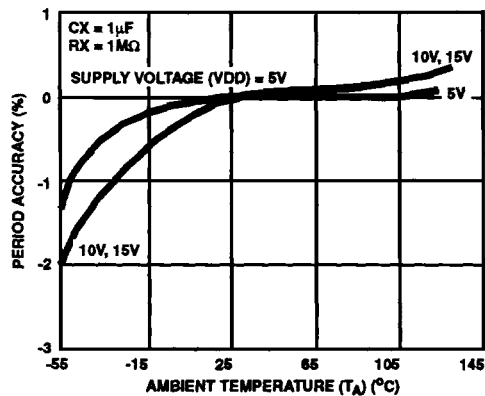
FIGURE 14. TYP. ASTABLE OSCILLATOR Q, \bar{Q} PERIOD ACCURACY vs AMBIENT TEMPERATURE (ULTRA LOW FREQ.)
