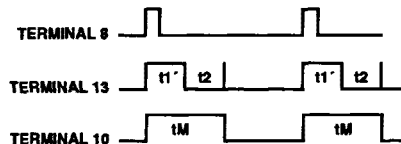
FIGURE 30. MONOSTABLE WAVEFORMS
