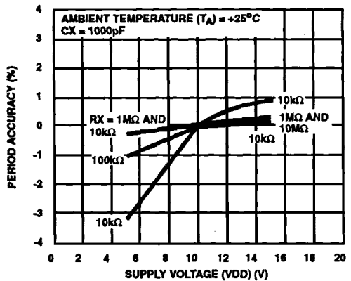
FIGURE 13. TYP. ASTABLE OSCILLATOR Q, \bar{Q} PERIOD ACCURACY vs SUPPLY VOLTAGE
