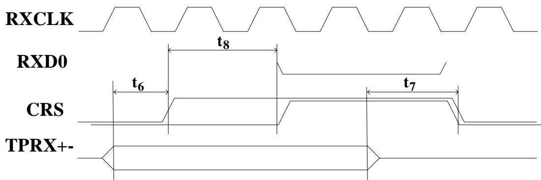
Figure 14. SNI Reception Cycle Timing
