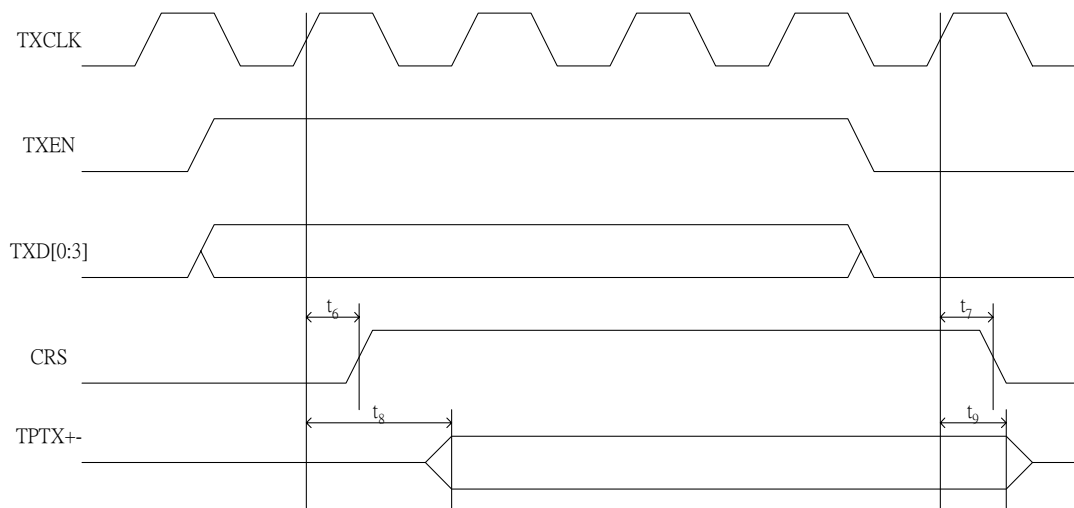
Figure 8. MII Transmission Cycle Timing
