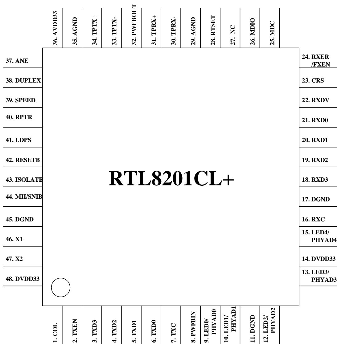
Figure 2. Pin Assignments
