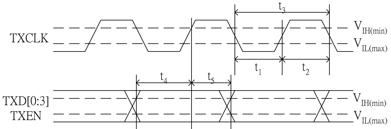
Figure 7. MII Transmission Cycle Timing
