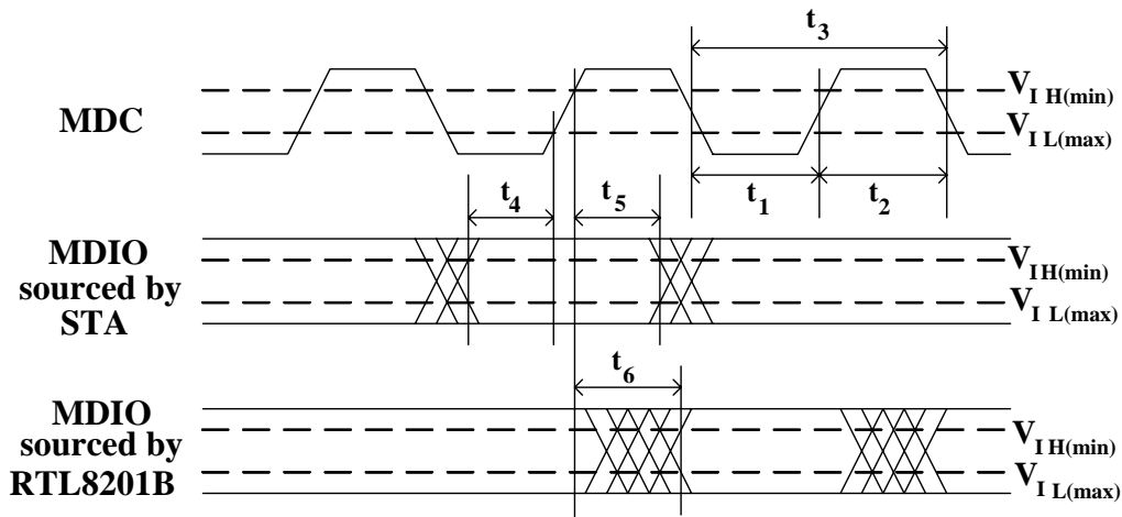
Figure 15. MDC/MDIO Timing
