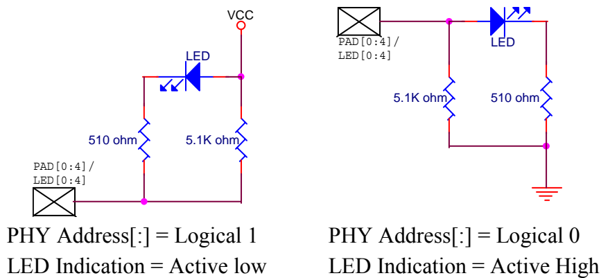
Figure 5. LED and PHY Address Configuration
