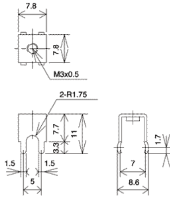
取付穴参考図 Processing reference figure
