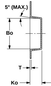
SECTION B-B
