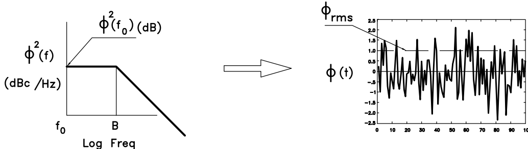
Figure 38. PLL with Integrated VCO Phase Noise & Jitter
