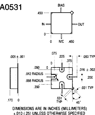
CA0531
