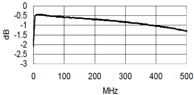
Insertion Loss
