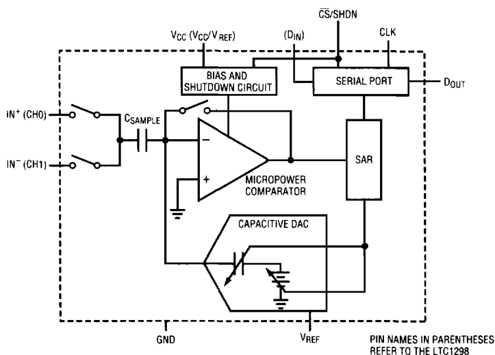
Block Diagram
