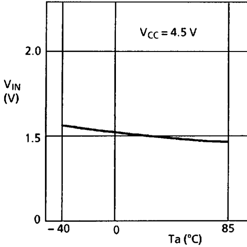
1.8 Input voltage V_{IN} — Ambient temperature T_a
