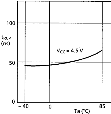
2.6 Recall pulse width t_{RCP} — Ambient temperature T_a
