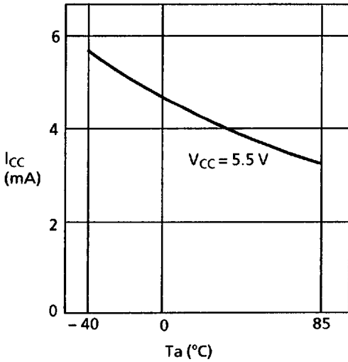
1.1 Operating current consumption I_{CC} — Ambient temperature T_a
