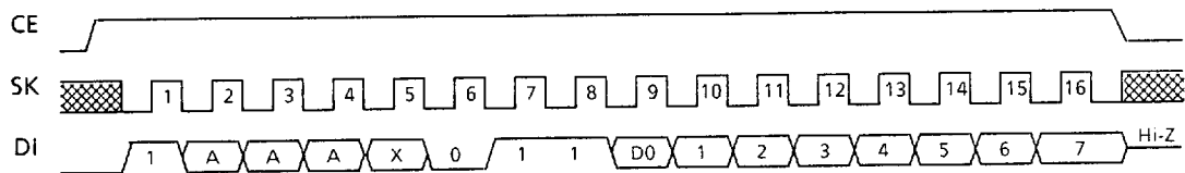
Figure 9 Write mode timing
