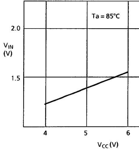
1.9 Input voltage V_{IN} — Power supply voltage V_{CC}
