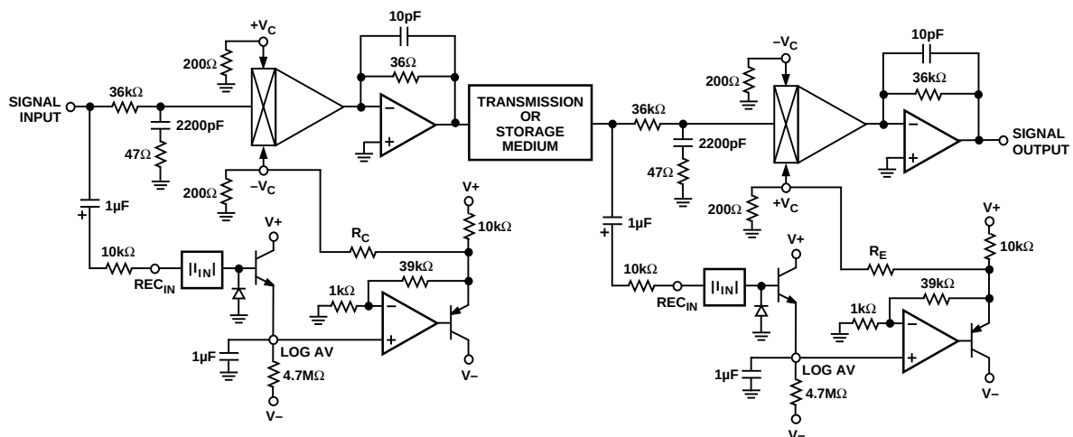
Figure 10. Companding Noise Rejection System
