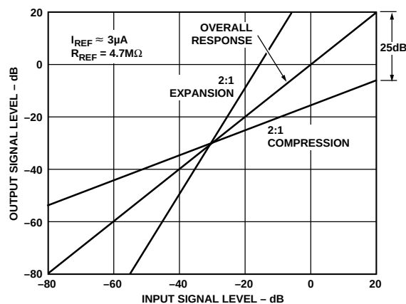
Figure 11. Companding Noise Reduction with 2:1 Compression/Expansion Ratio
