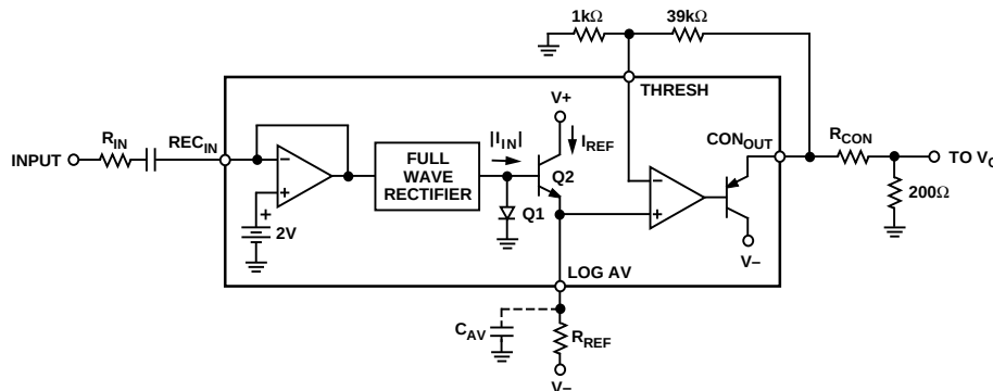
Figure 3. Level Detector
