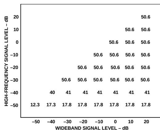
c. V_{THRESH} at V–
