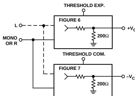
a. Control Circuit
