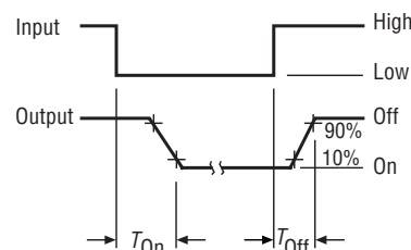
Figure 3 - Output Turn-on and Turn-off Timing
