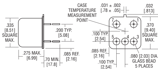
Figure 7 - Outline Dimensions
