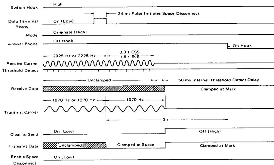
FIGURE 7 — INITIATE DISCONNECT
