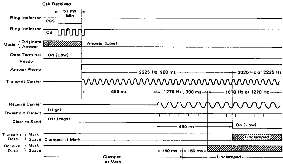
FIGURE 4 — ANSWER MODE
