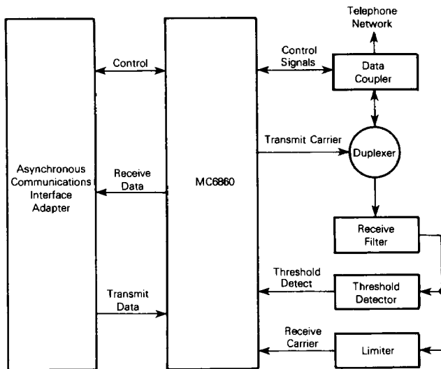
FIGURE 1 — TYPICAL MC6860 SYSTEM CONFIGURATION
