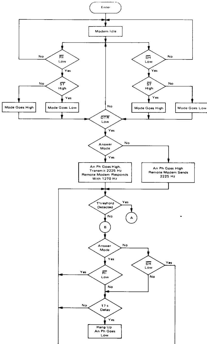
FIGURE 11 — FLOW DIAGRAM
