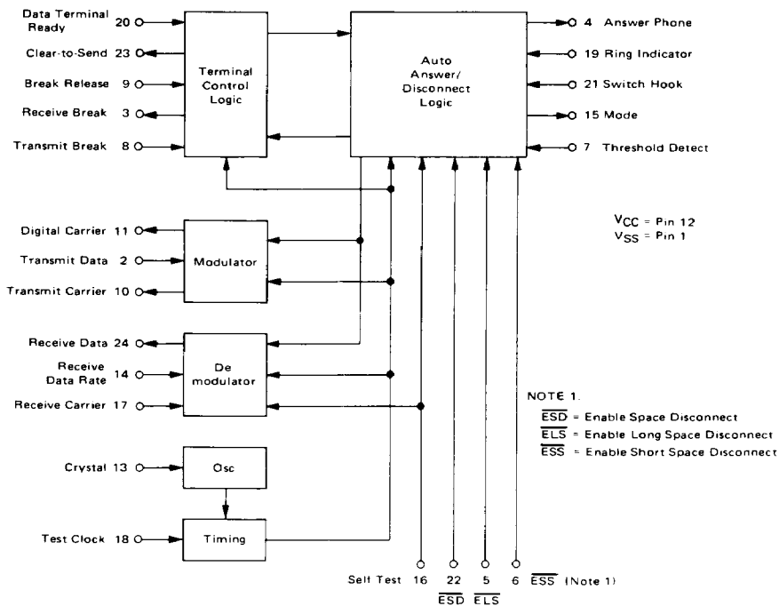
FIGURE 3 — BLOCK DIAGRAM
