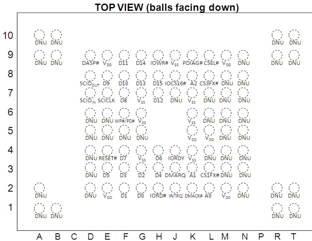
Figure 3.1: Pin Assignments for 91-Ball PBGA
