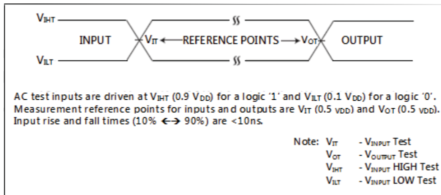
Figure 4: AC Input/Output Reference Waveforms
