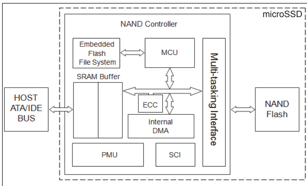
Figure 2-1: PATA microSSD Block Diagram
