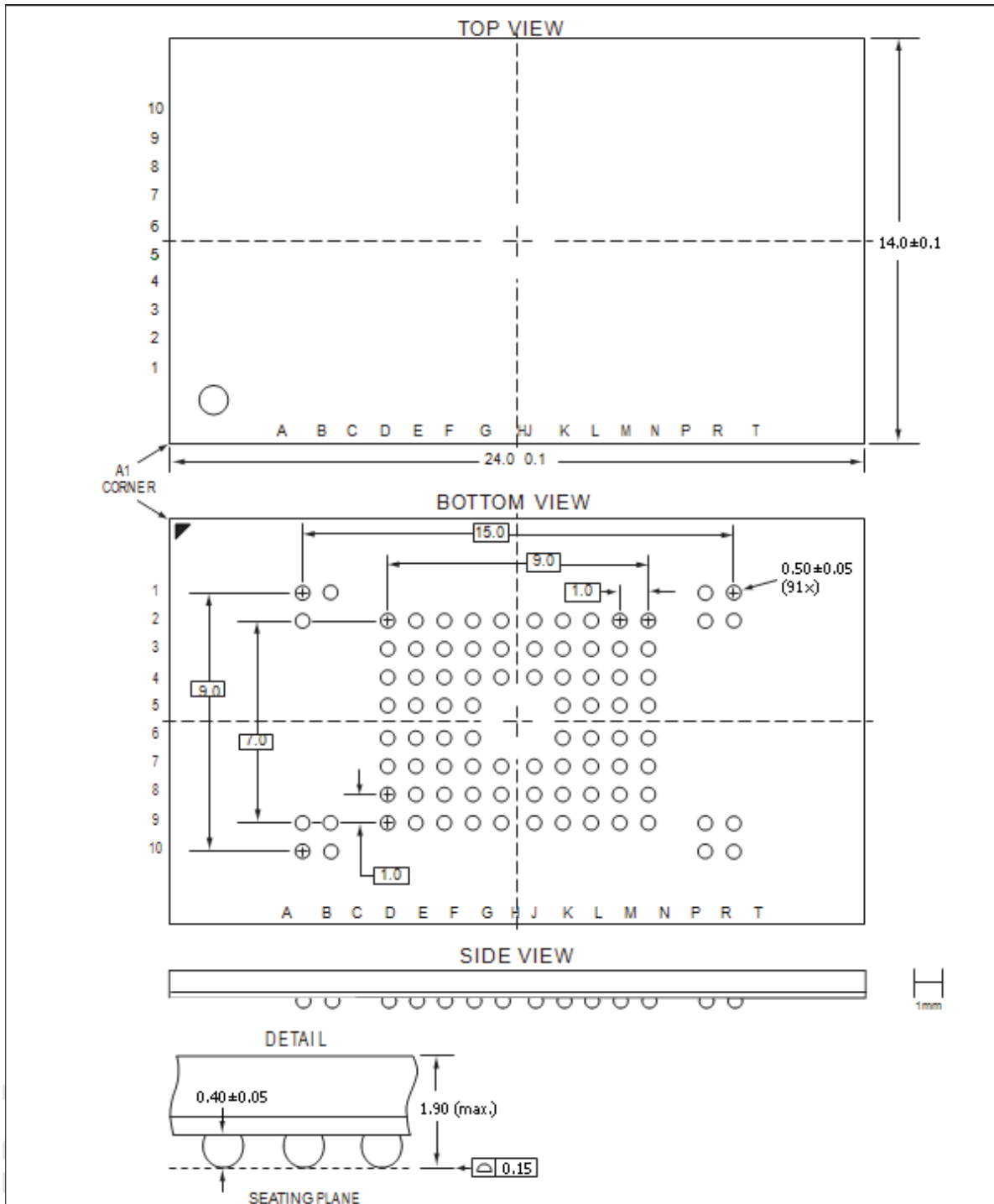
Figure 6: microSSD 91-Ball, Plastic Ball Grid Array (PBGA) MicroSSD Package Code: PBG
