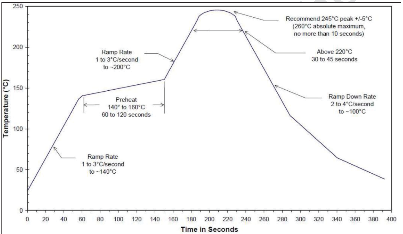
Figure 5: Soldering Reflow Profile
