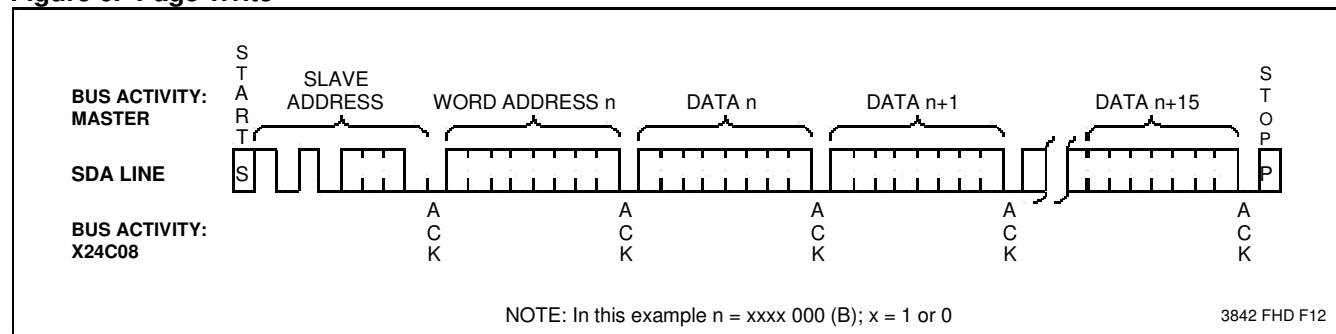
Figure 6. Page Write
