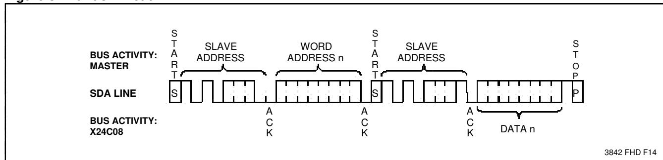
Figure 8. Random Read
