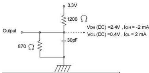
(Fig. 1) DC Output Load Circuit
