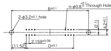
PCB Mounting Dimensions Applicable PCB Thickness=1.6±0.19mm
