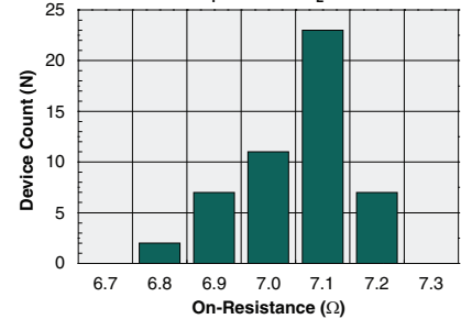
Typical On-Resistance Distribution (N=50, I_F=0.5\text{mA} , I_L=75\text{mA} )
