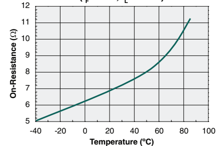
Typical On-Resistance vs. Temperature ( I_F=1\text{mA} , I_L=50\text{mA} )
