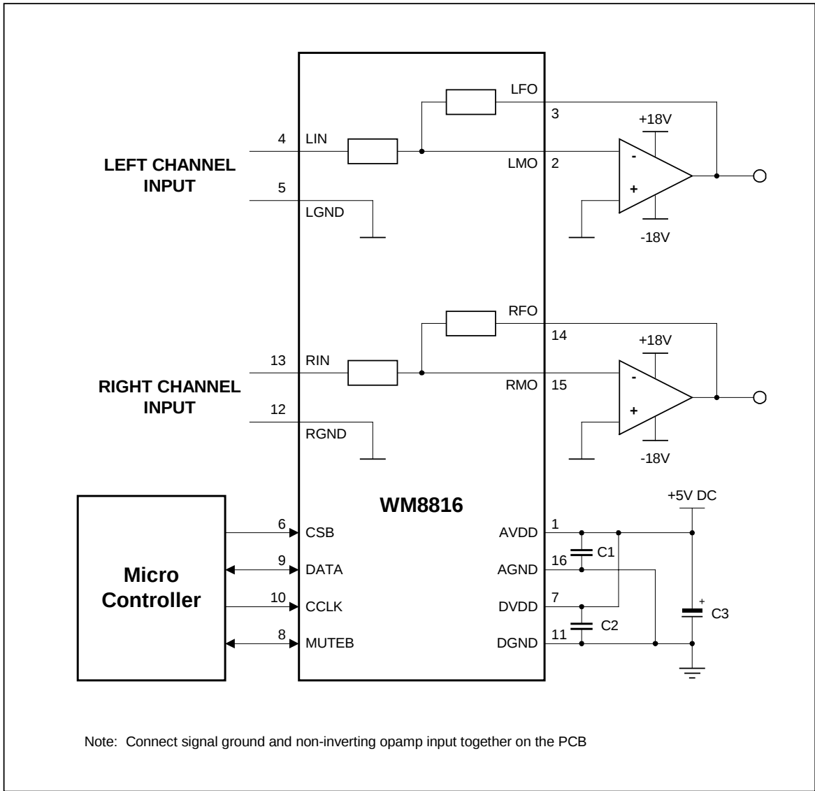
Figure 5 Typical Application
