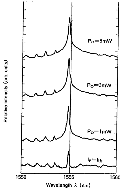
Fig. 6 Emission spectrum under modulated operation
