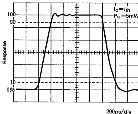
Fig. 10 Pulse response waveform
