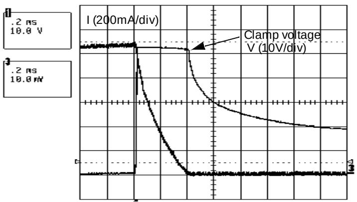
Figure17- Inductive Switching
