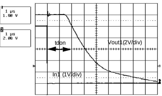
Figure18- Turn on Delay
