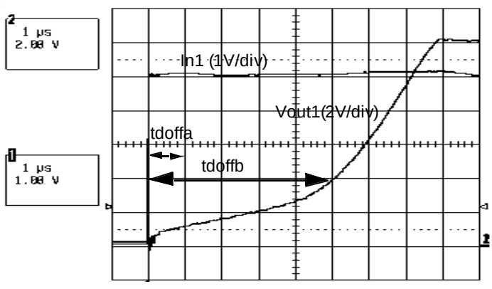
Figure19- Turn off Delay
