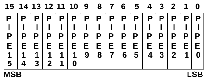
Figure 21. The PIPE Register (PIPE)
