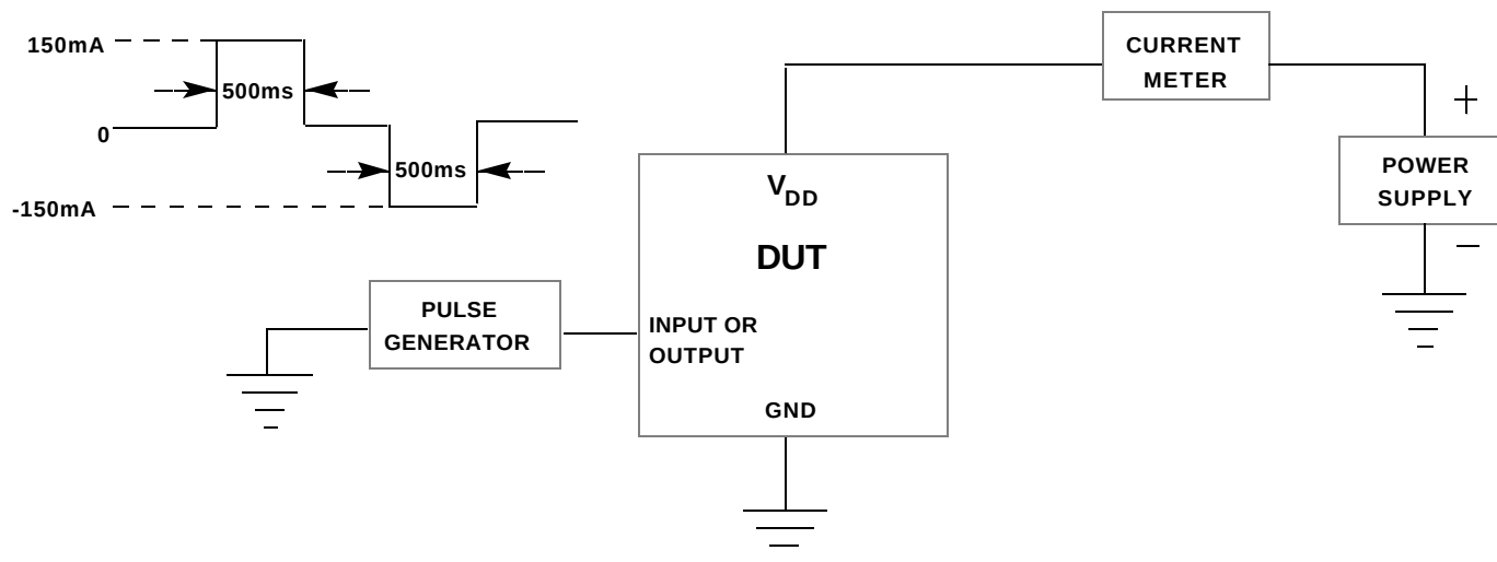
Figure 43. Latchup Test
