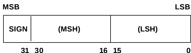
Figure 31b. Double 32-Precision Fixed-Point Data
