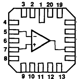
20-Pad LCC (Top View)
