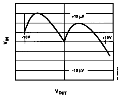
Typical Precision Op Amp Gain Linearity
