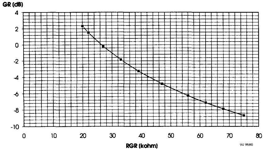
Figure 14. Typical adjustment range of the receive gain
