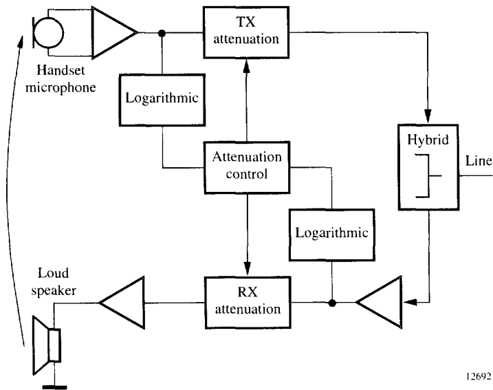
Figure 6. Basic voice-switch system
