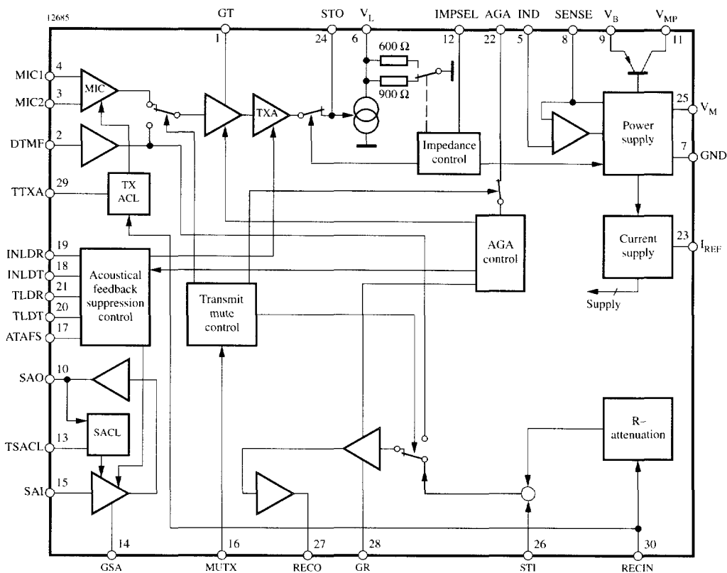
Figure 1. Block diagram
