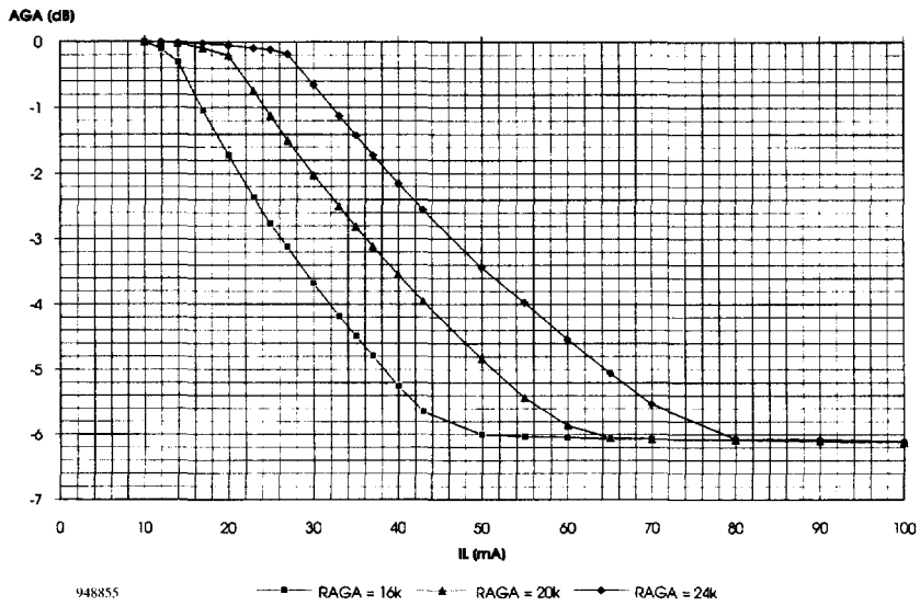
Figure 15. Typical AGA characteristic
