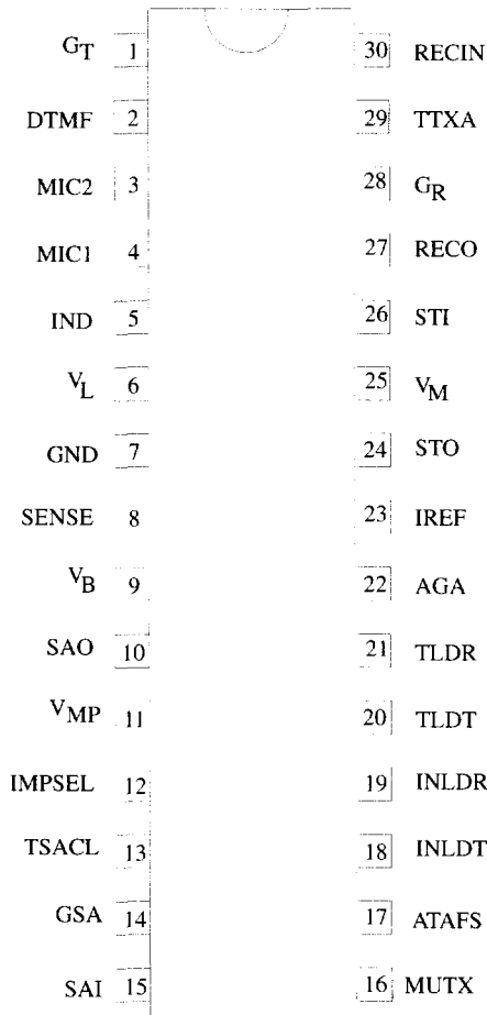
Figure 3. Pinning
