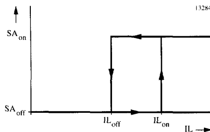
Figure 10. Threshold of speaker amplifier
