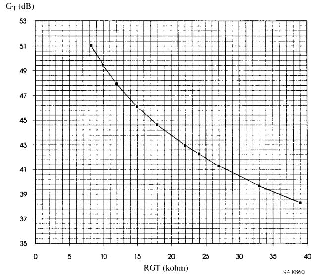
Figure 13. Typical adjustment range of the transmit gain
