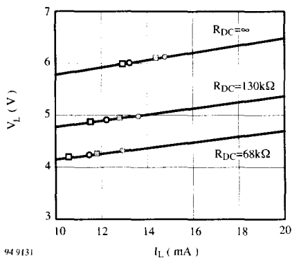
Figure 10. Threshold of speaker amplifier
