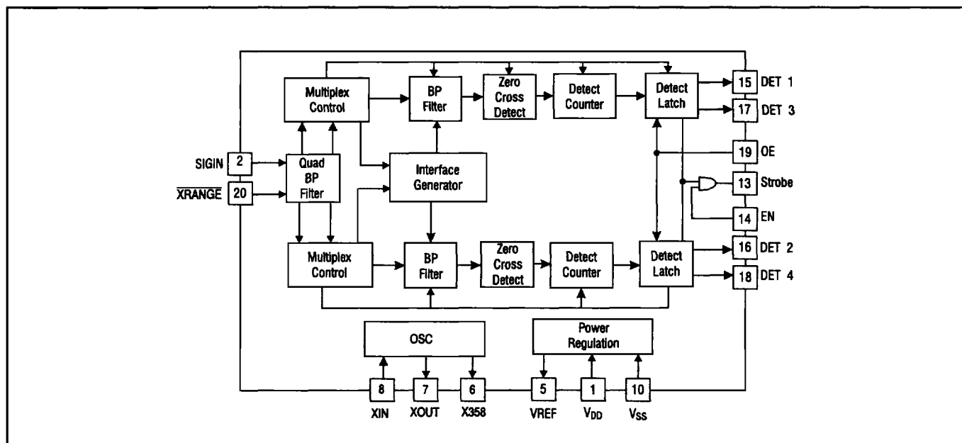
Figure 2 Block Diagram
