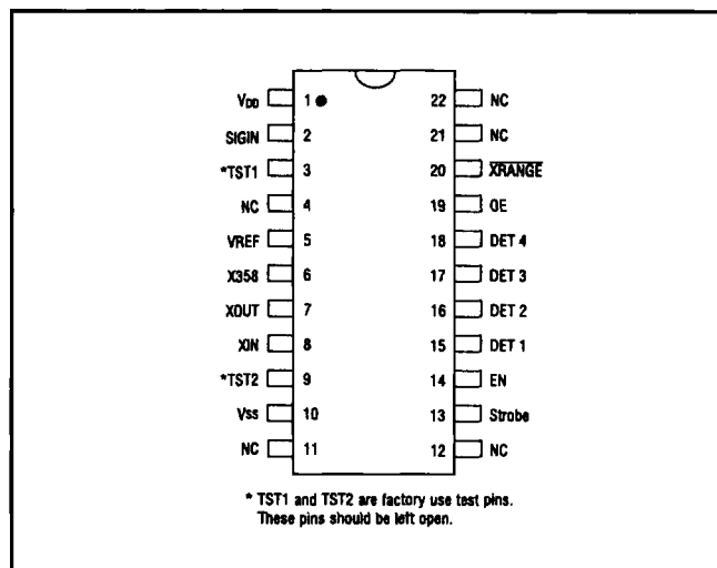
Figure 1 Pin Diagram
