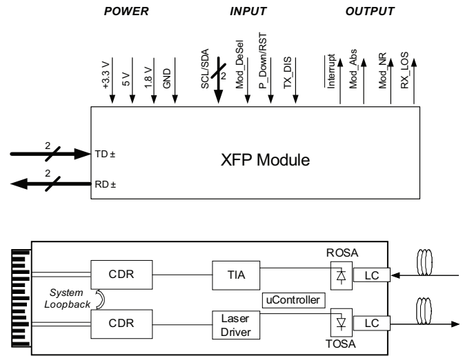
Figure 2. Application schematics
