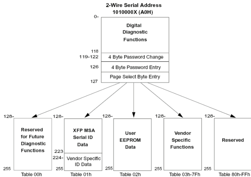
Figure 5. XFP 2-wire serial digital diagnostic memory map
