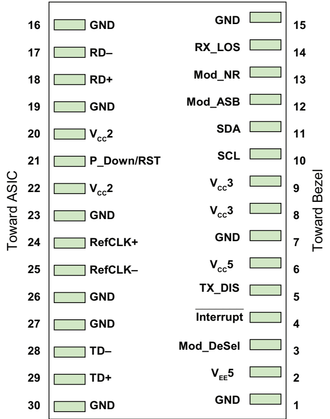
Figure 3. Transceiver pin assignments on host board
