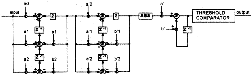
Fig 2. Tone Detector Block Diagram
