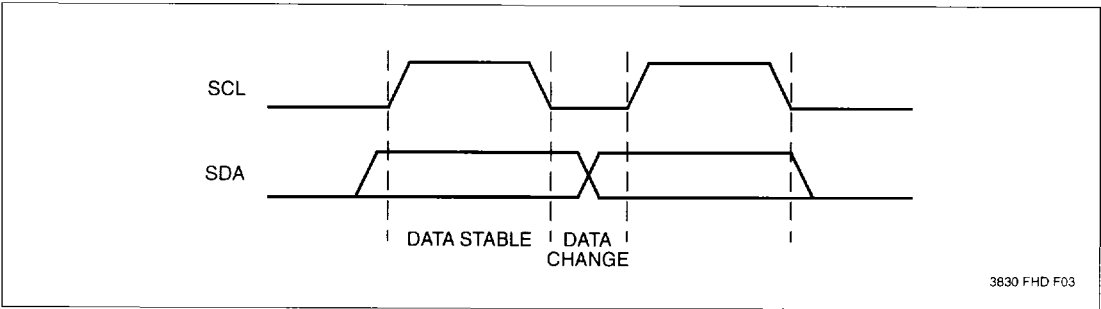
Figure 1. Data Validity
