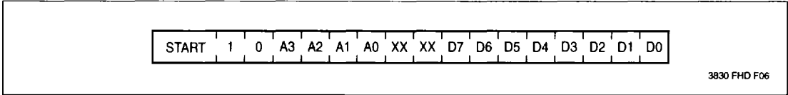
Figure 4. Read Sequence
