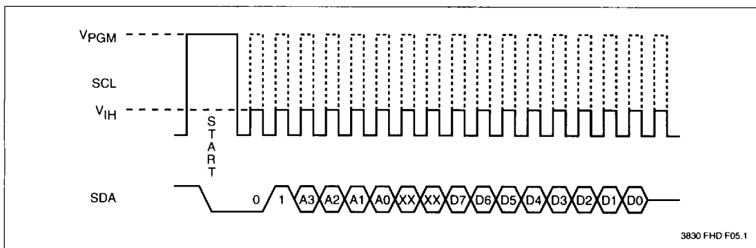
Figure 3. Programming Sequence
