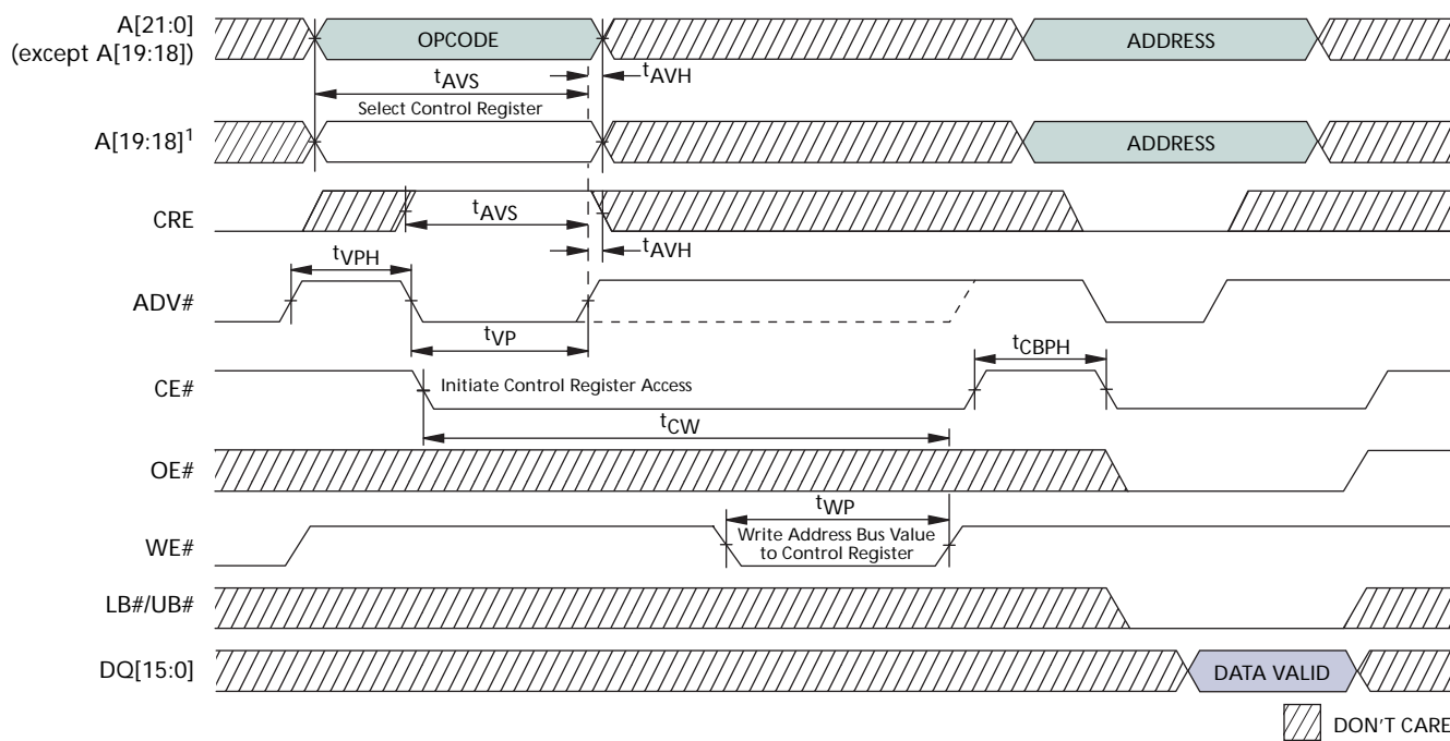
Figure 12: Configuration Register WRITE, Asynchronous Mode Followed by READ ARRAY
