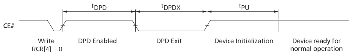
Figure 29: DPD Entry and Exit Timing
