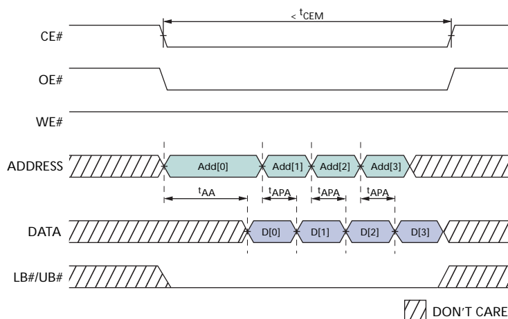
Figure 7: Page Mode READ Operation (ADV# LOW)
