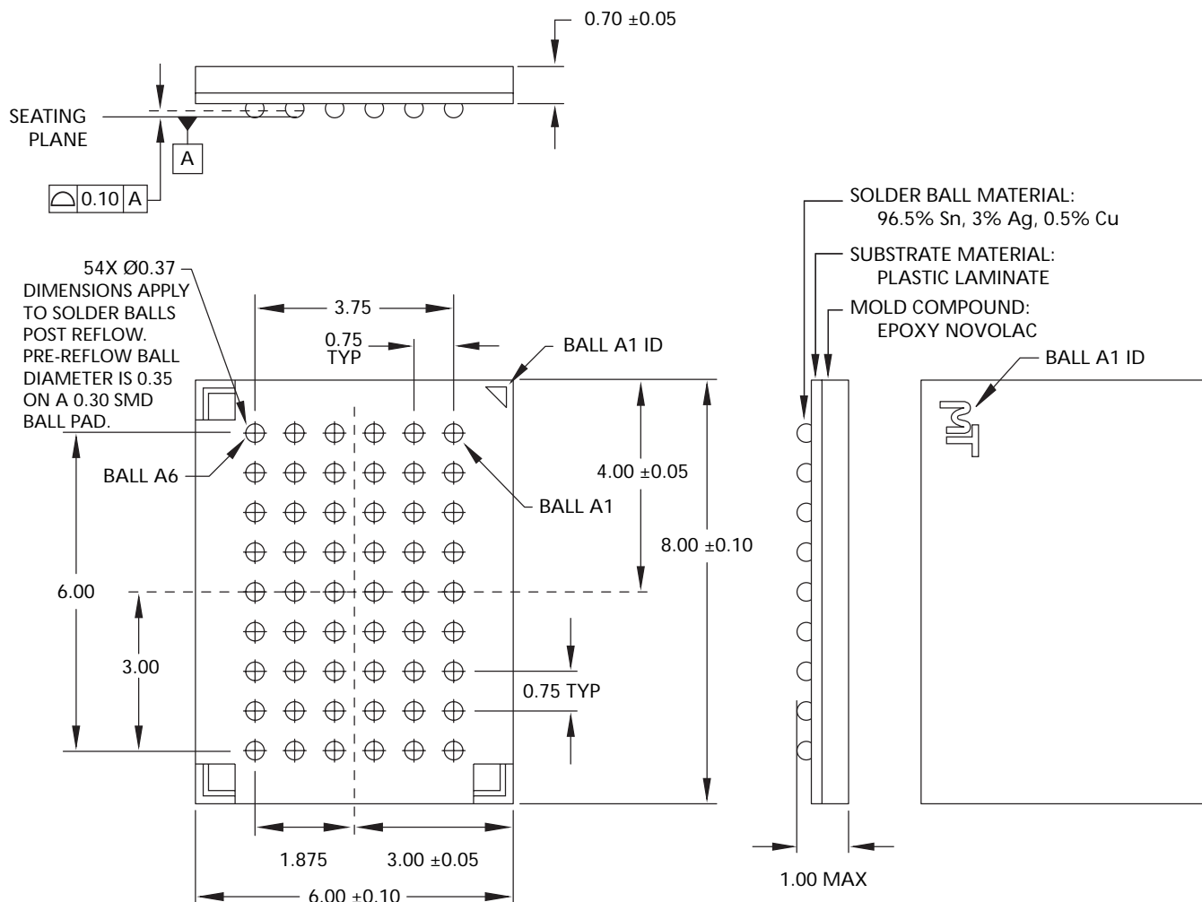
Figure 56: 54-Ball VFBGA
