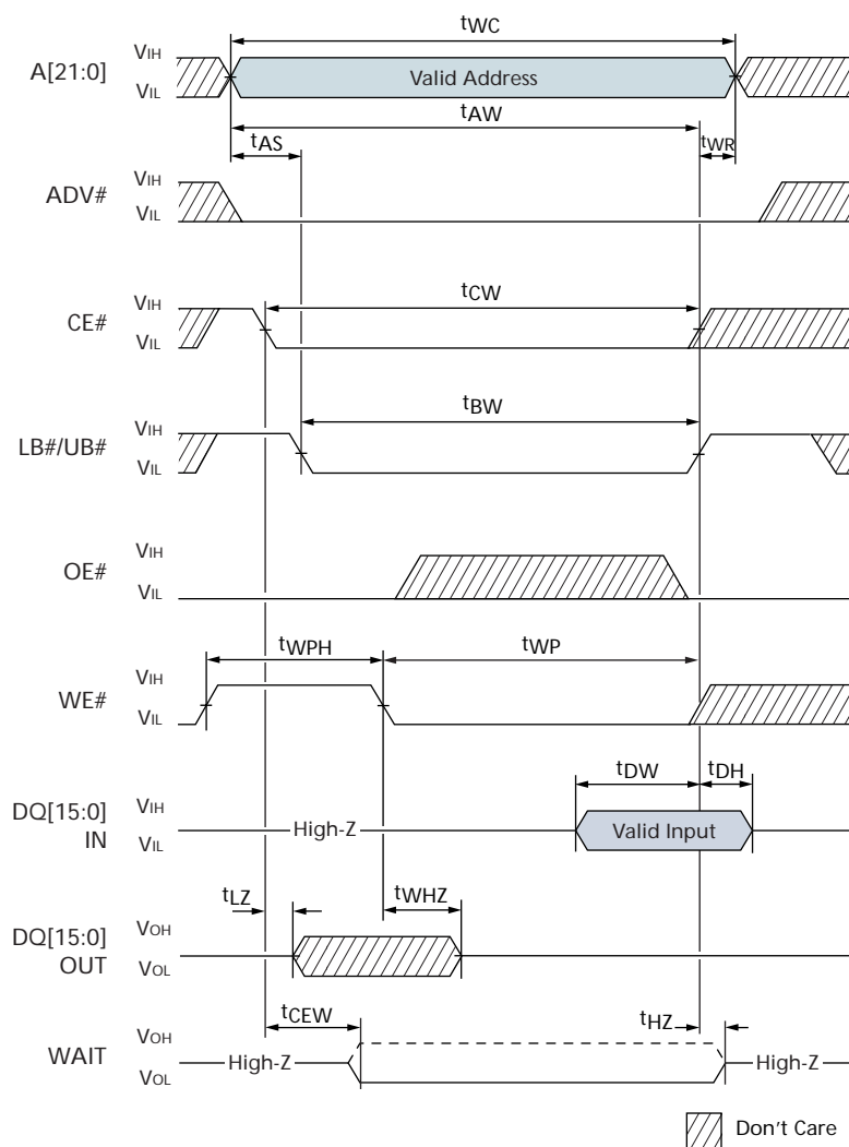
Figure 40: LB#/UB#-Controlled Asynchronous WRITE
