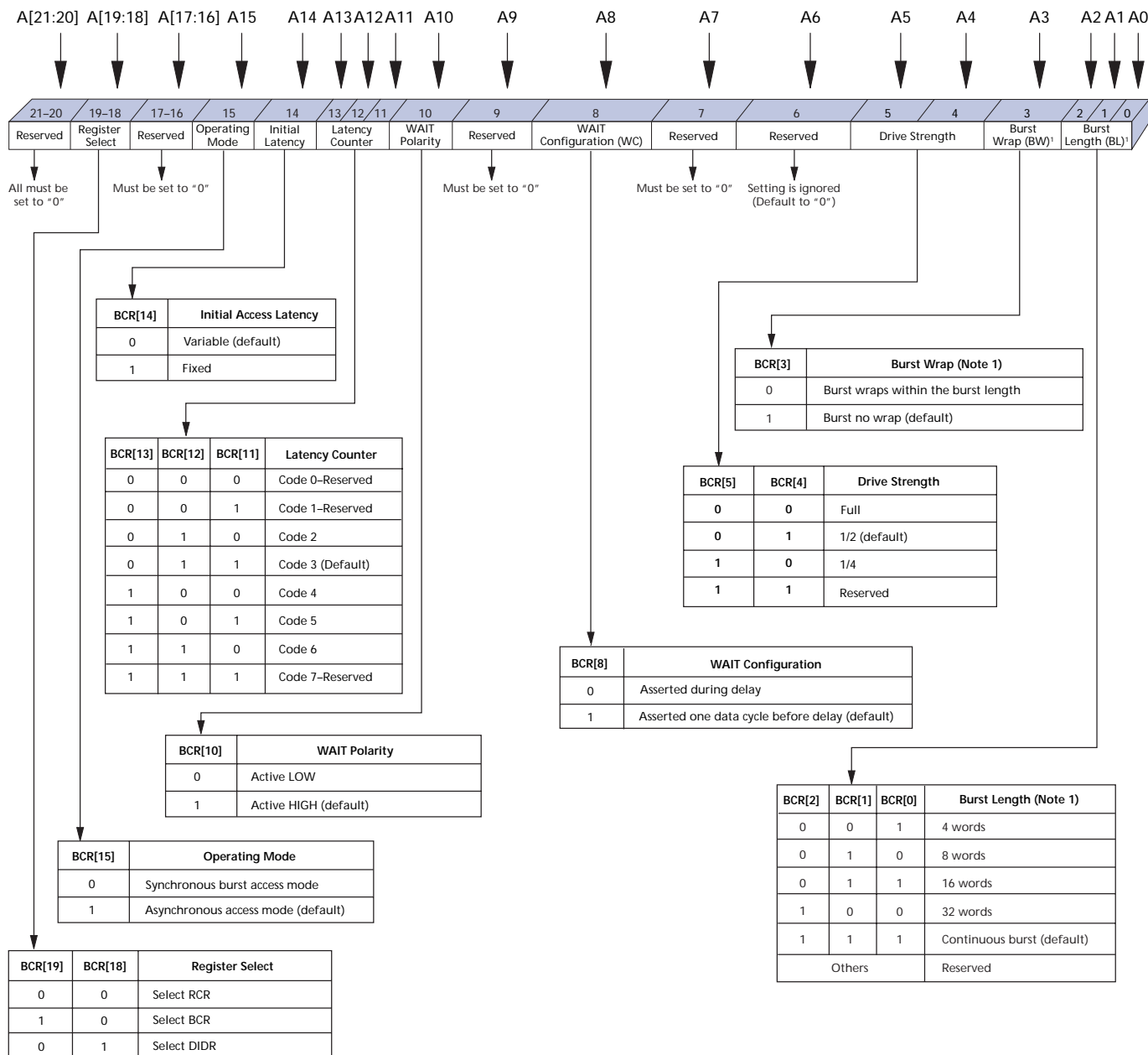
Figure 18: Bus Configuration Register Definition
