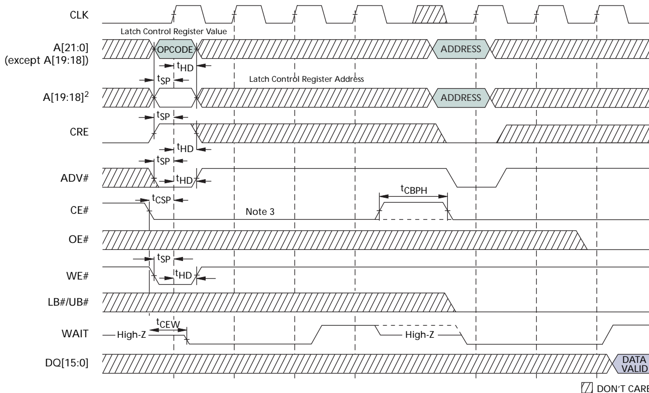
Figure 13: Configuration Register WRITE, Synchronous Mode Followed by READ ARRAY Operation
