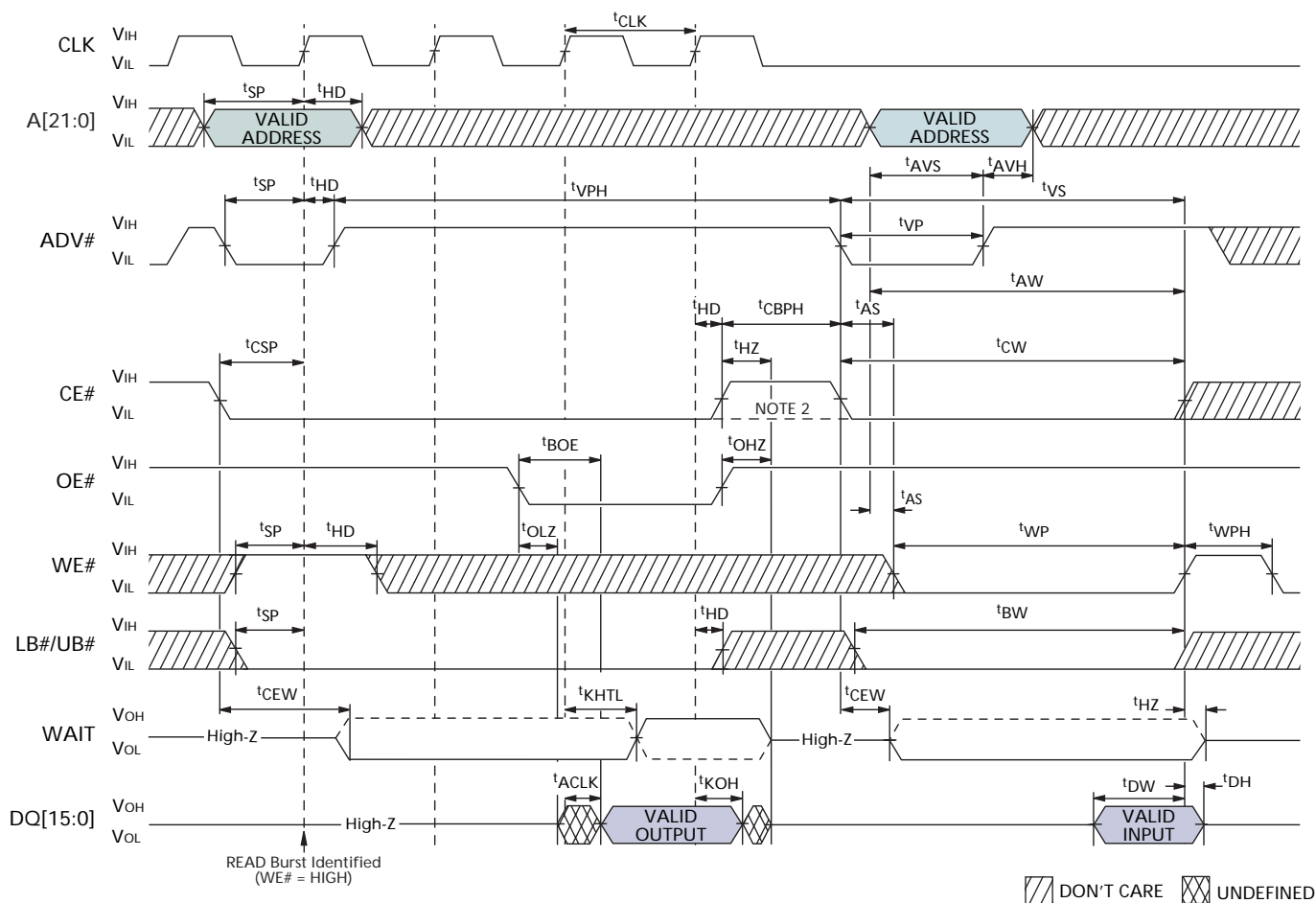
Figure 53: Burst READ Followed by Asynchronous WRITE Using ADV#
