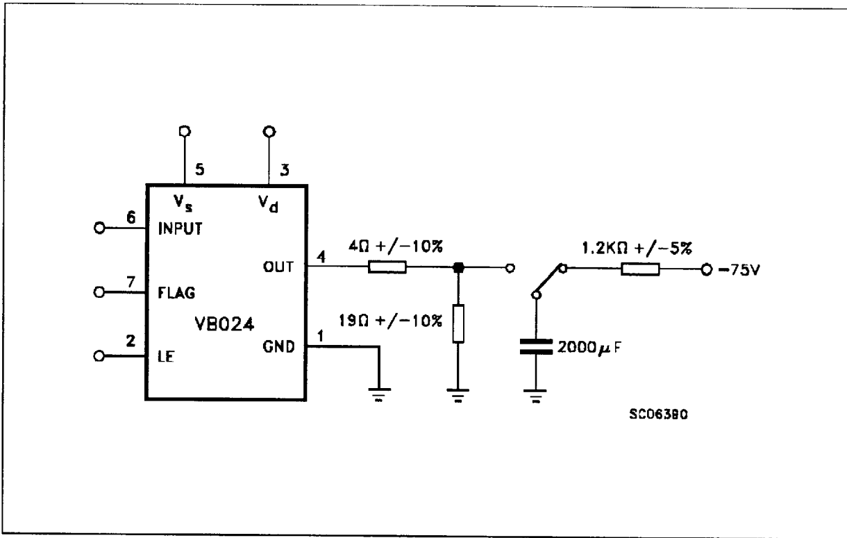
FIGURE 5: Negative Transients Test Circuit
