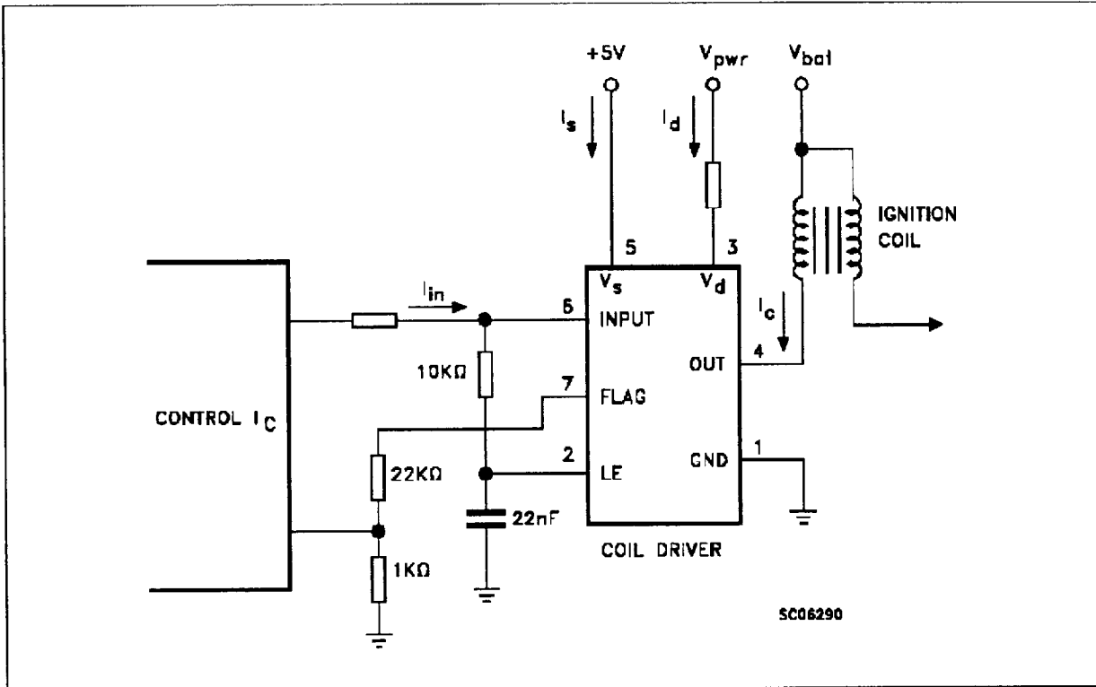
FIGURE1: Application Circuit
