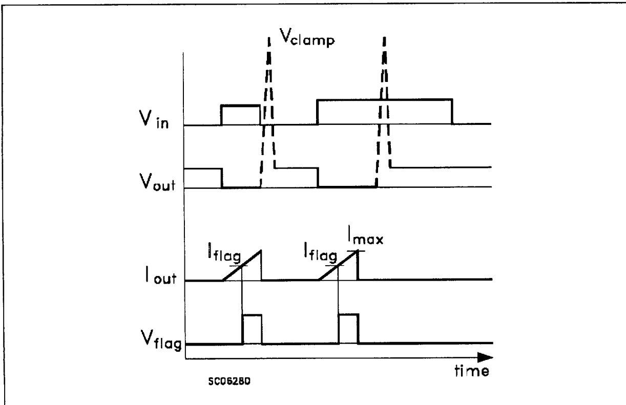
FIGURE2: Switching Waveforms
