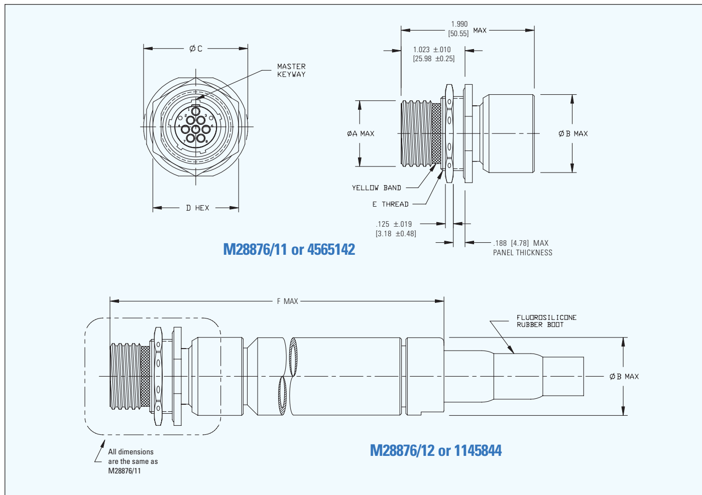
Dimension Table, Jam Nut Mounting Receptacles
