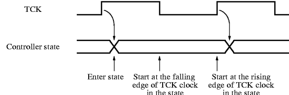
Fig 3. Operation timing of controller state
