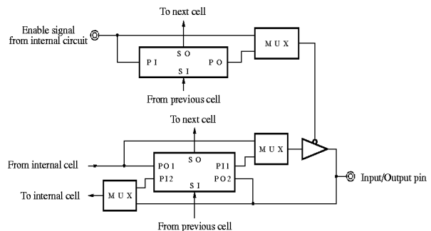
Fig7. I/O type cell
