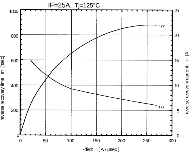
Reverse recovery time characteristics vs. -di/dt
