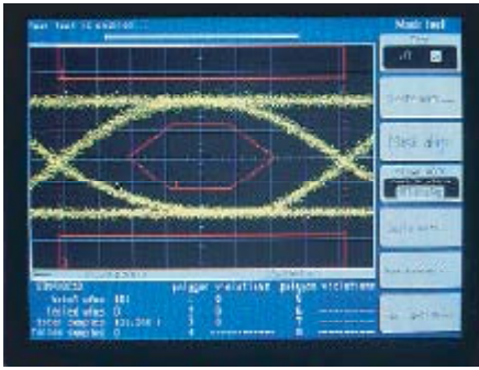
Testing an eye-opening mask to ensure CCITT/ANSI compliance.
