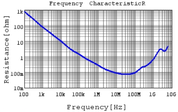
GCM188R72A103KA37 R DC0V, 25degC
