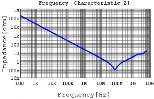
GCM188R72A103KA37 |Z| DC0V, 25degC
