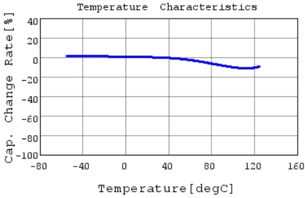
GCM188R72A103KA37 C-Temp. capchange, DC0.0V,
