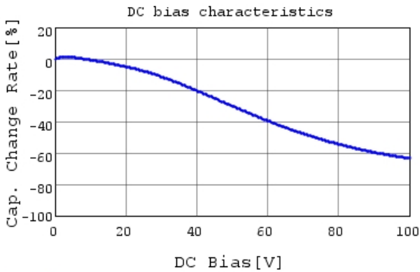
GCM188R72A103KA37 C-DC bias capchange, 25.0c
