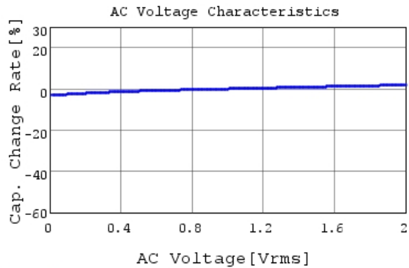
GCM188R72A103KA37 C-AC Voltage capchange, DC
