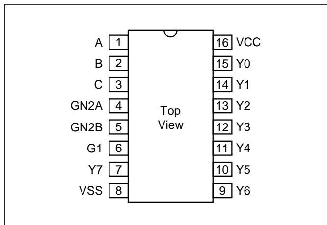
Figure 5: DIL Pin Out
