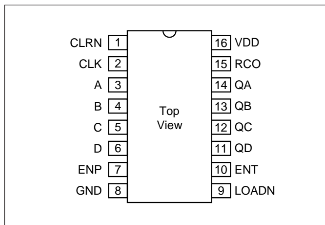
Figure 8: DIL Pin Out
