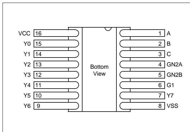
Figure 6: Flatpack Pin Out
