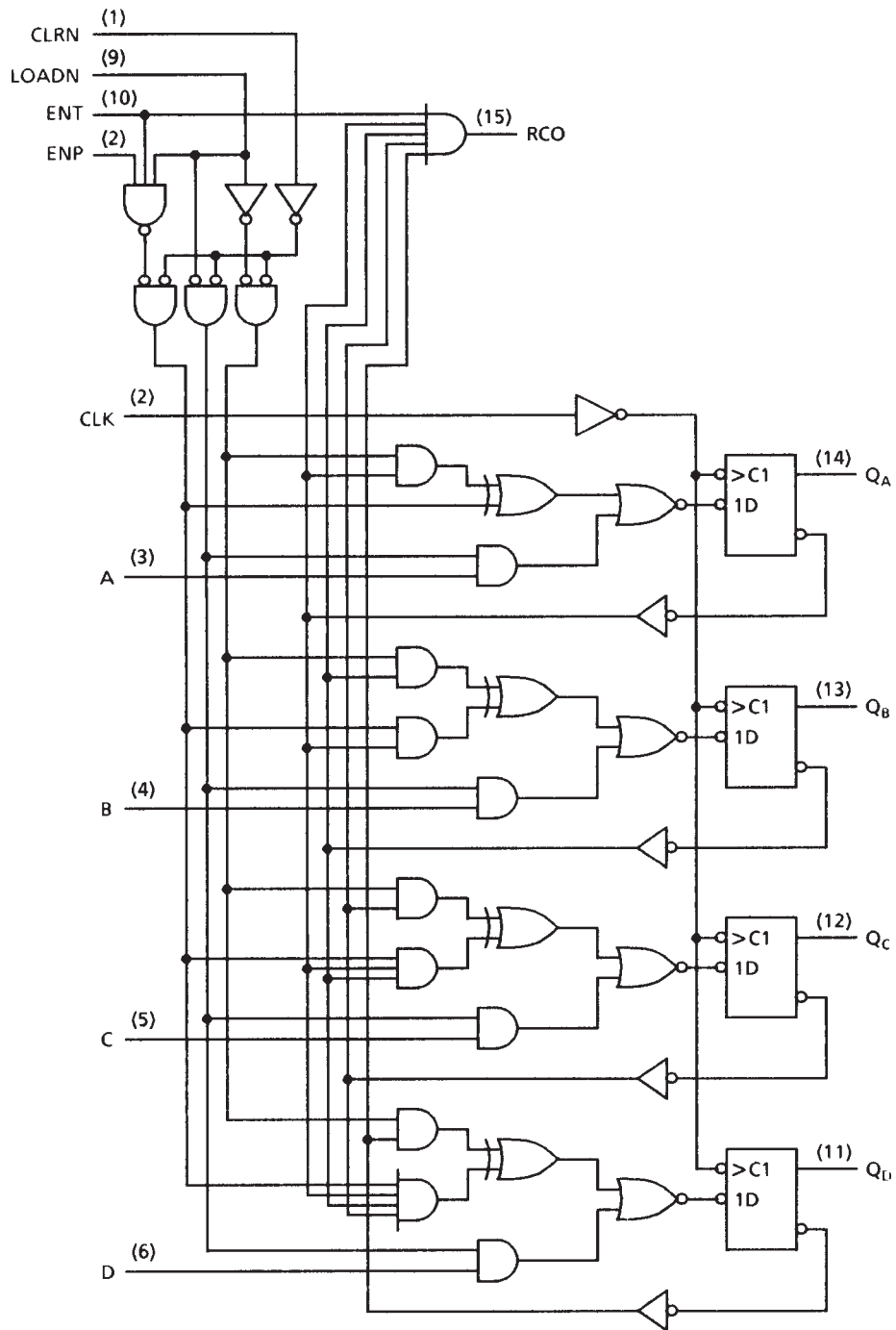
Figure 10: Logic Diagram
