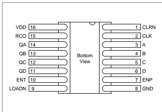
Figure 9: Flatpack Pin Out
