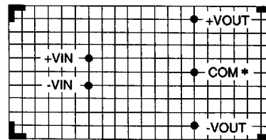
BOTTOMVIEW - "B" Package Option
