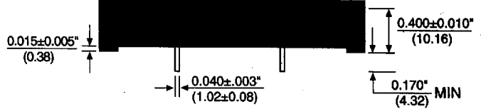
SIDEVIEW - "B" Package Option
