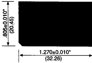
TOPVIEW - "A" Package Option
