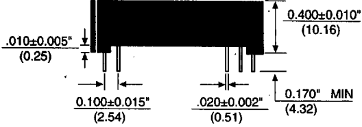
SIDEVIEW - "A" Package Option
