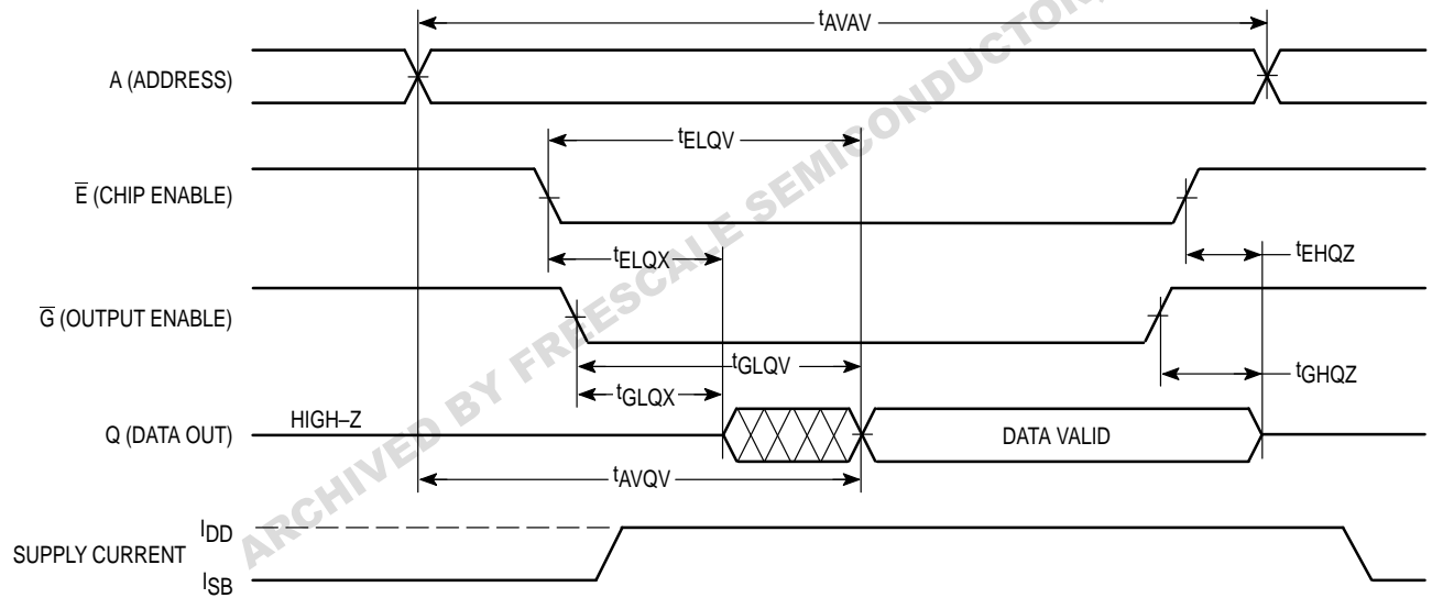
READ CYCLE 2 (See Note 4)
