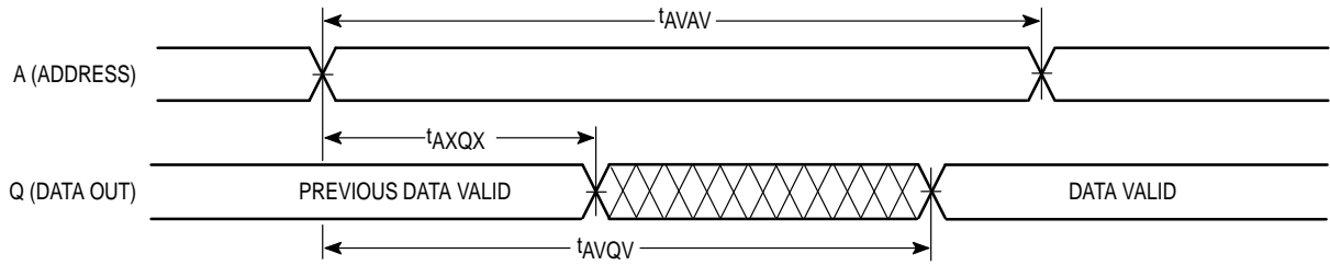
READ CYCLE 1 (See Note 8)
