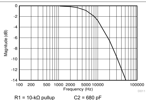
Figure 8-5. Low-Pass Filtering
