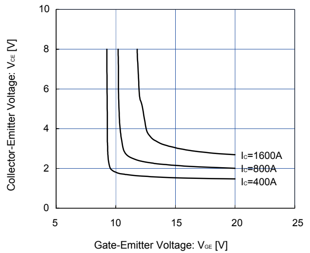
Collector-Emittor voltage vs. Gate-Emittor voltage T_j = 25^\circ\text{C} / chip
