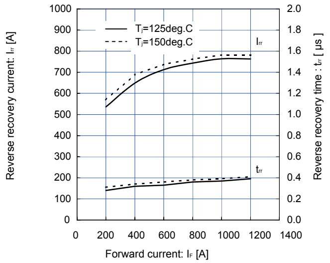
Reverse Recovery Characteristics (typ.) V_{CC}=900\text{V} , V_{GE}=\pm 15\text{V} , R_{\theta gn}=2.4\Omega
