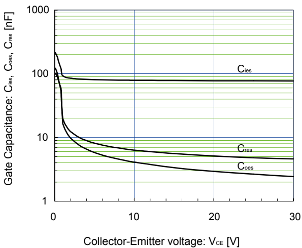
Gate Capacitance vs. Collector-Emittor Voltage V_{GE} = 0\text{V} , f = 1\text{MHz} , T_j = 25^\circ\text{C}
