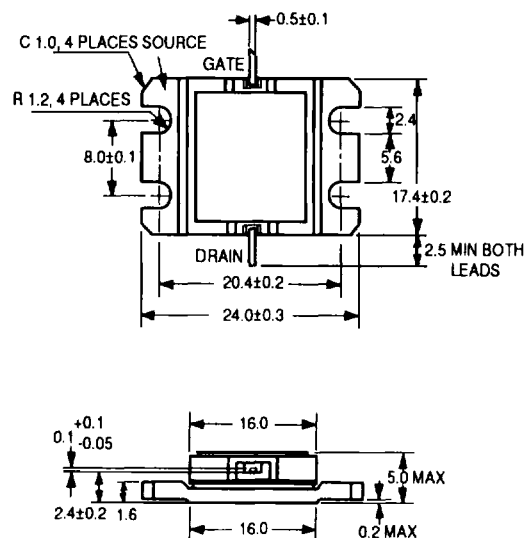
PACKAGE OUTLINE T-65
