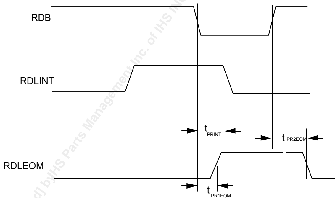
Figure 47 - Receive Data Link DMA Interface Output Timing Diagram
