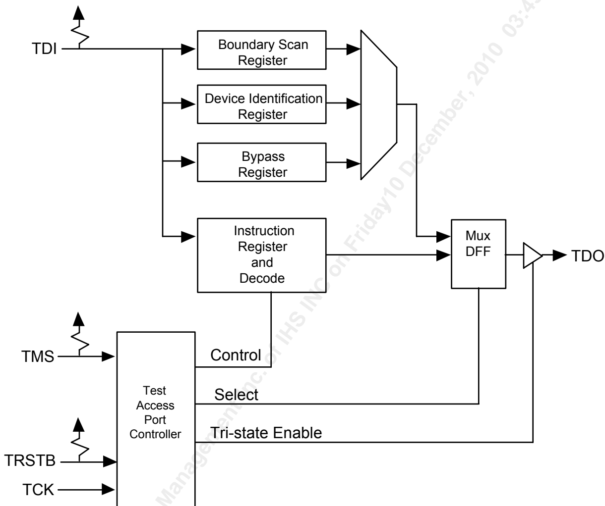
Figure 32 - Boundary Scan Architecture
