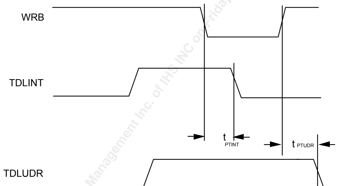
Figure 46 - Transmit Data Link DMA Interface Output Timing Diagram
