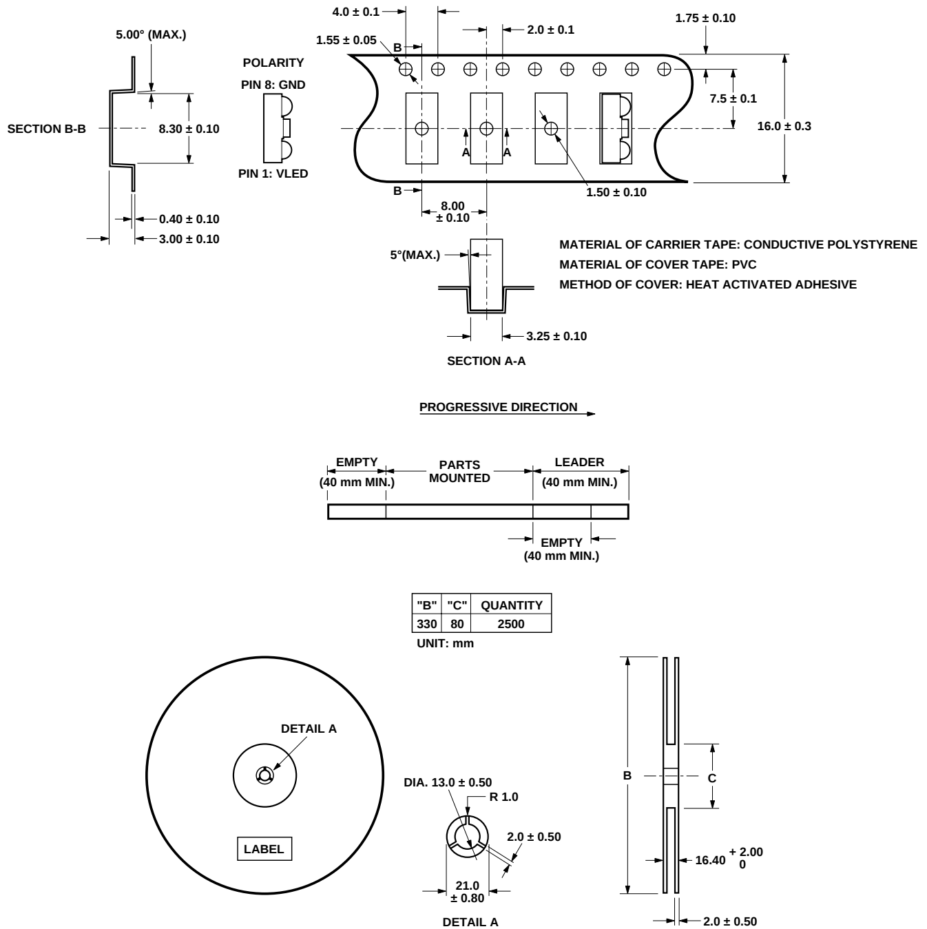
Figure 14. Tape and reel dimensions.
