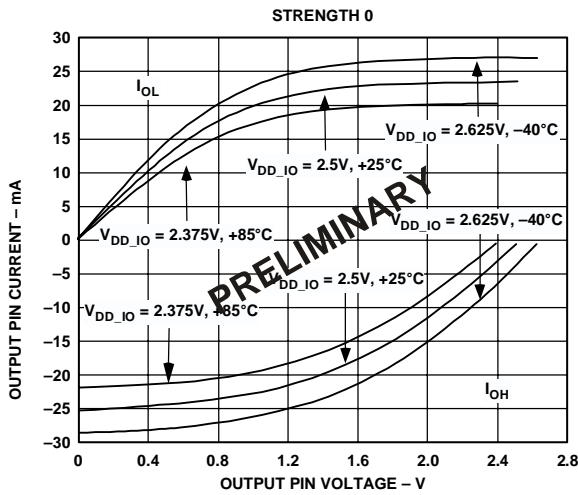
Figure 23. Typical Drive Currents at Strength 0
