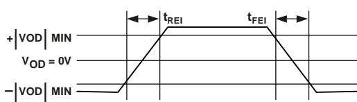
Figure 21. Link Ports—Differential Input Signals Transition Time
