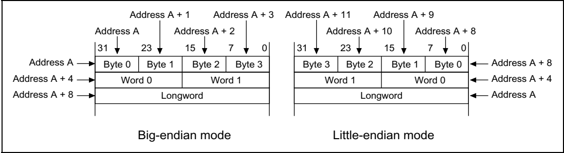
Figure 2.11 Byte, Word, and Longword Alignment
