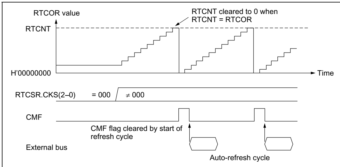
Figure 12.18 Auto-Refresh Operation
