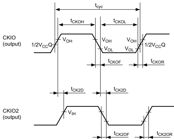
Figure 32.3 CKIO Clock Output Timing
