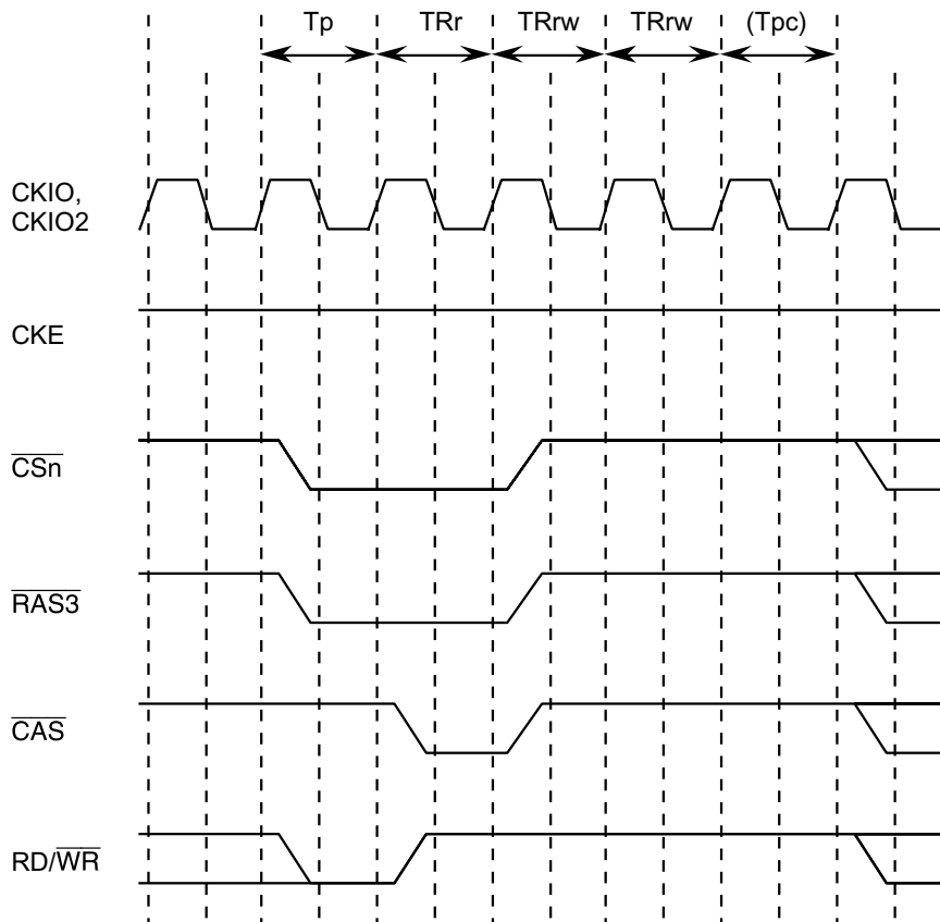
Figure 12.19 Synchronous DRAM Auto-Refresh Timing
