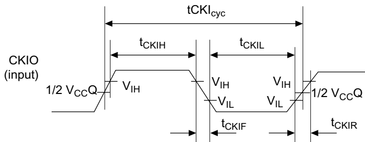
Figure 32.2 CKIO Clock Input Timing
