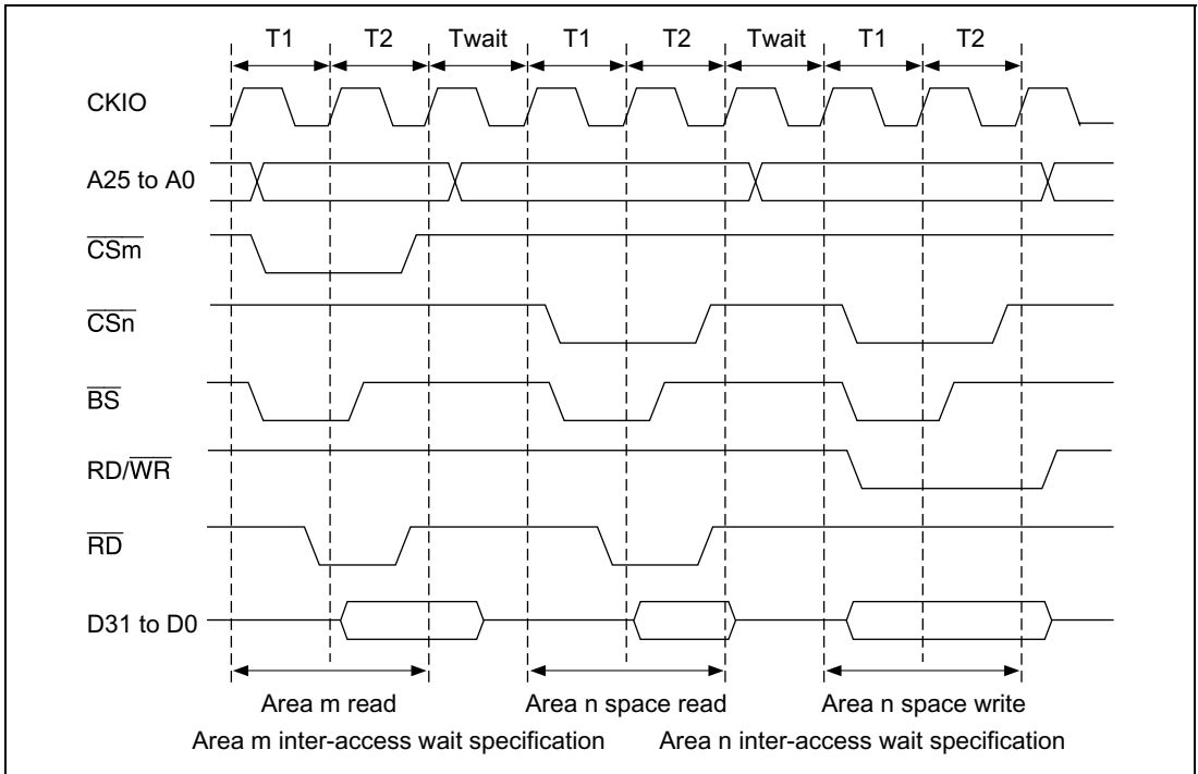
Figure 12.33 Waits between Access Cycles
