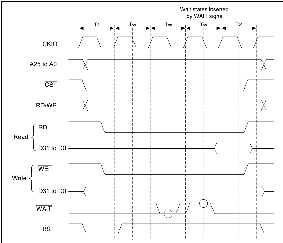
Figure 12.10 Basic Interface Wait State Timing (Wait State Insertion by \overline{\text{WAIT}} Signal \text{WAITSEL} = 1 )
