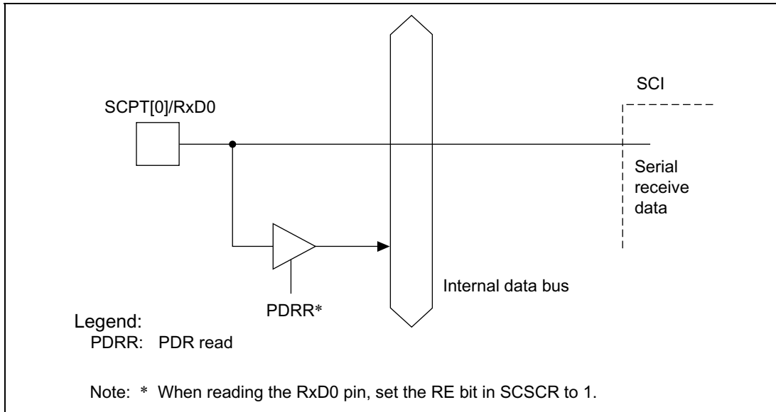
Figure 17.4 SCPT[0]/RxD0 Pin
