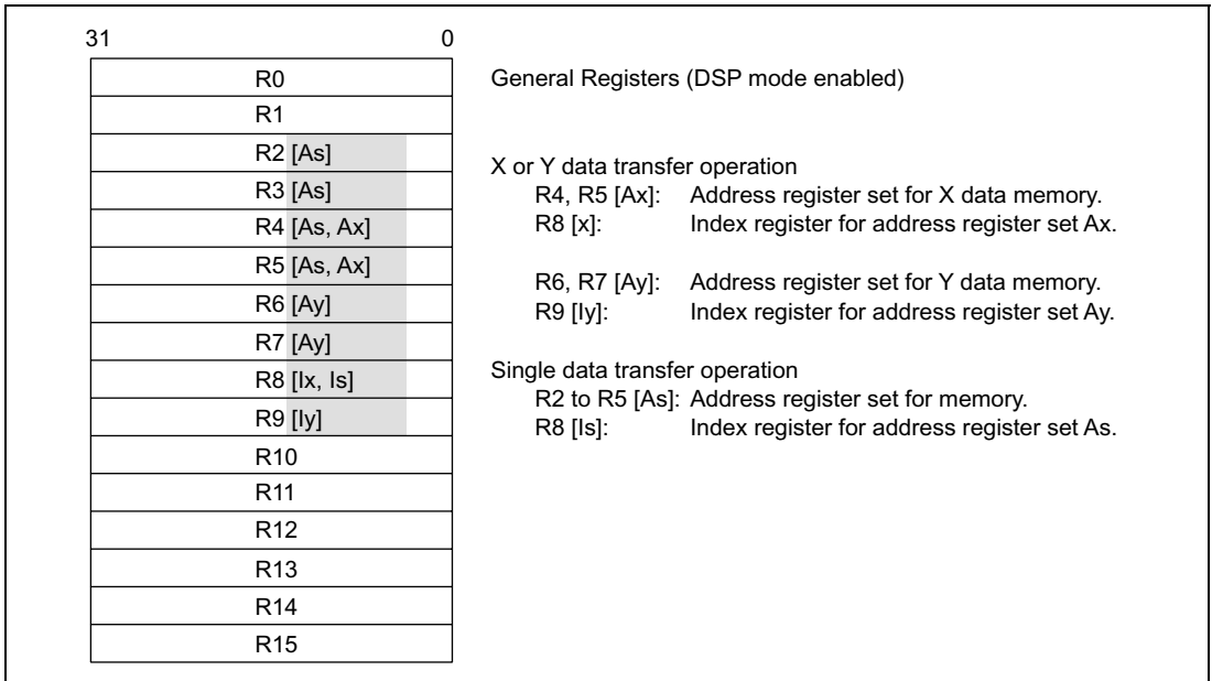
Figure 2.4 General Purpose Register (DSP Mode)
