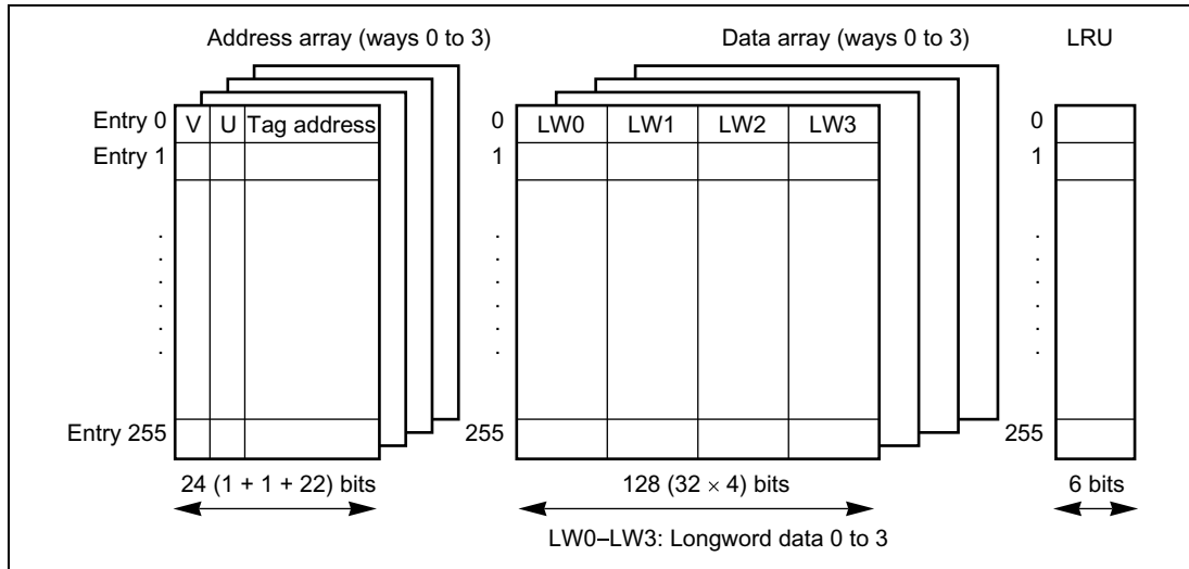
Figure 5.1 Cache Structure
