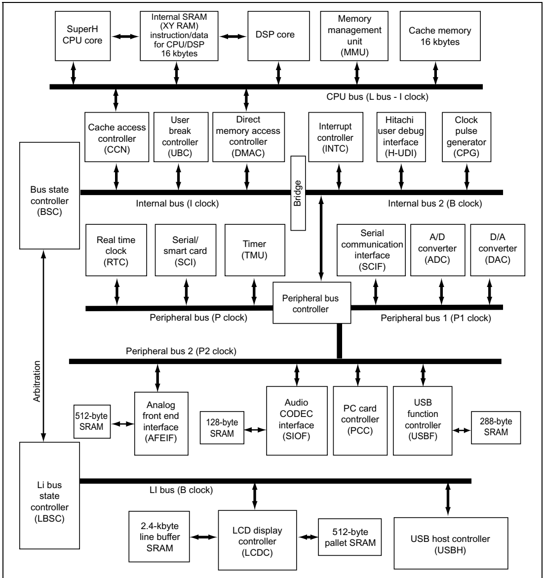
Figure 1.1 Block Diagram
