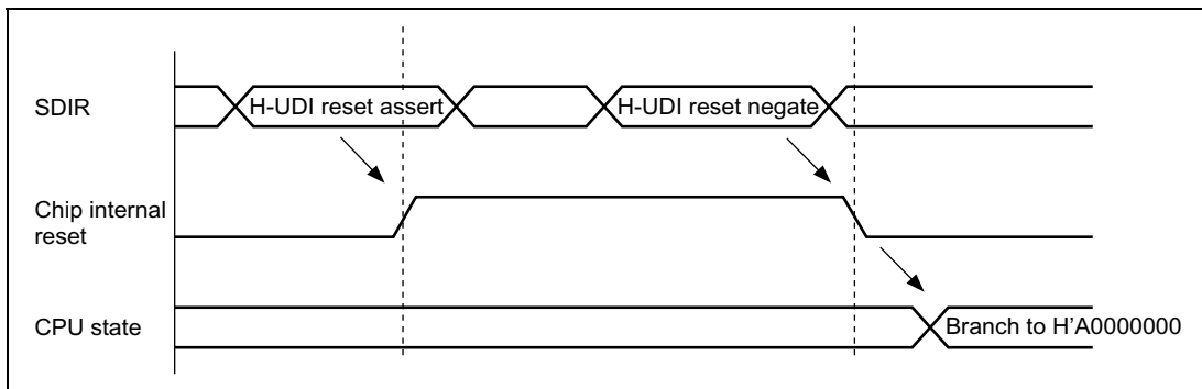
Figure 31.3 H-UDI Reset
