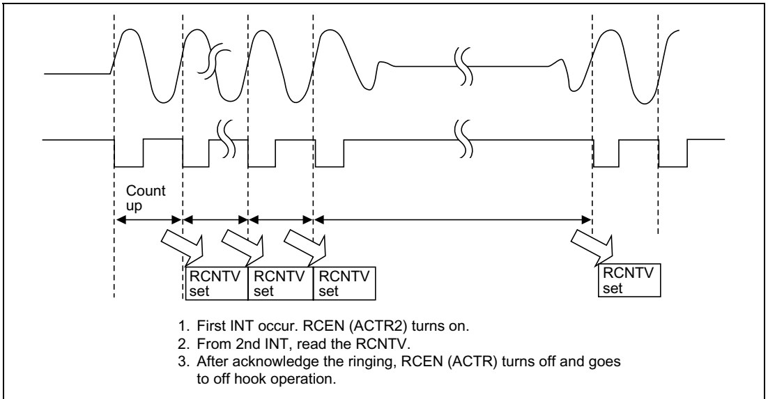
Figure 21.8 Ringing Detect Sequence
