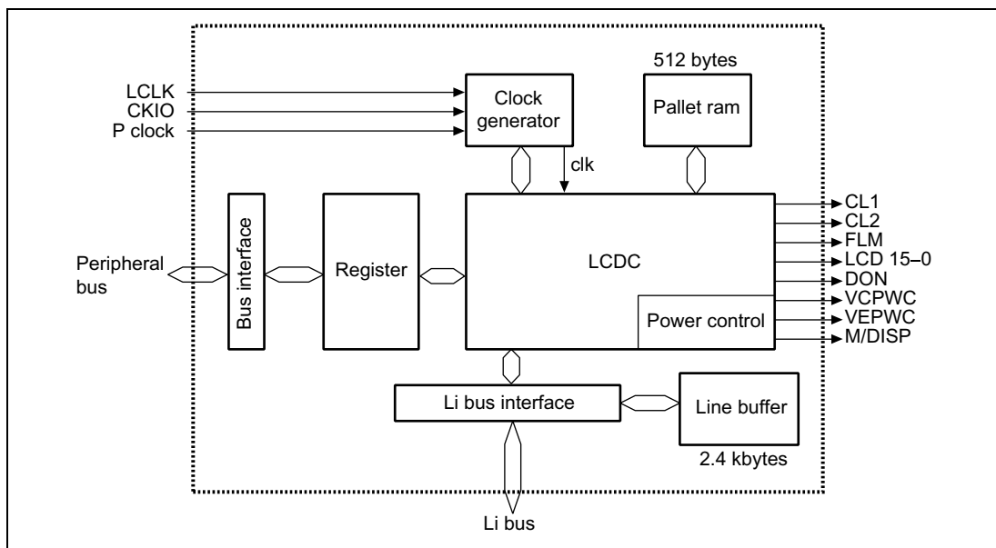
Figure 25.1 Block Diagram
