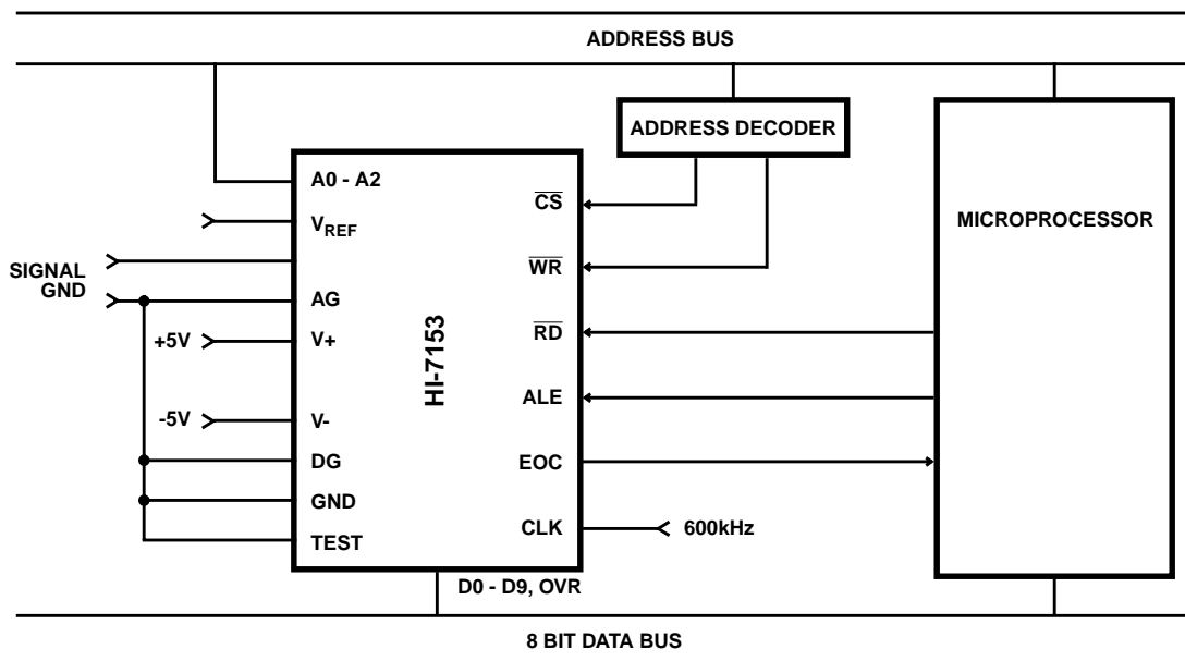
FIGURE 4. MULTI-CHANNEL DATA ACQUISITION SYSTEM
