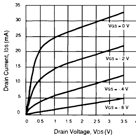
DC PERFORMANCE
