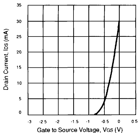
DRAIN CURRENT vs. GATE VOLTAGE (TYP)
