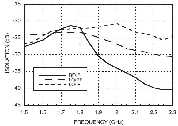
Single Channel: Isolation
