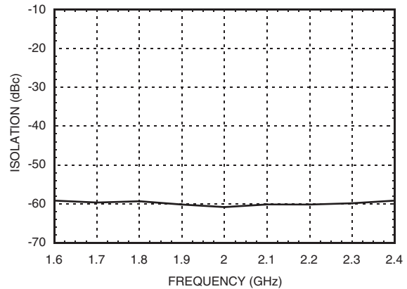
Dual Channel: LO1 to LO2 Isolation [2]
