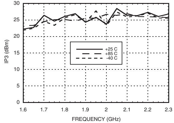
Single Channel: Input IP3 vs. Temperature
