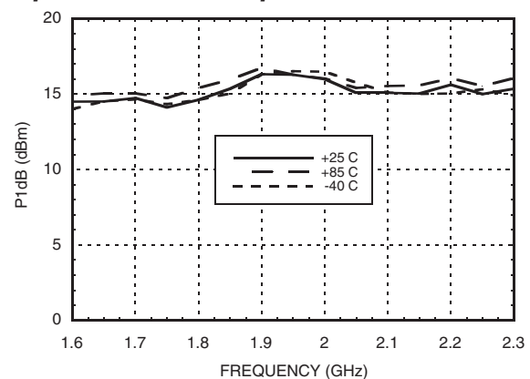
Single Channel: Input P1dB vs. Temperature
