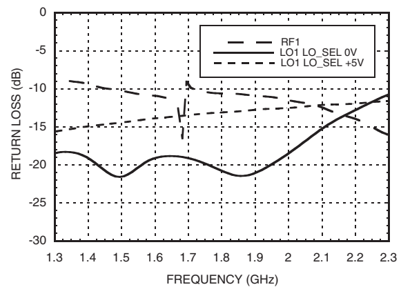
Single Channel: Return Loss
