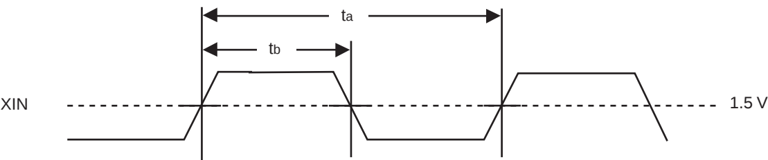
Input clock duty cycle (t DCI = t b /t a )
