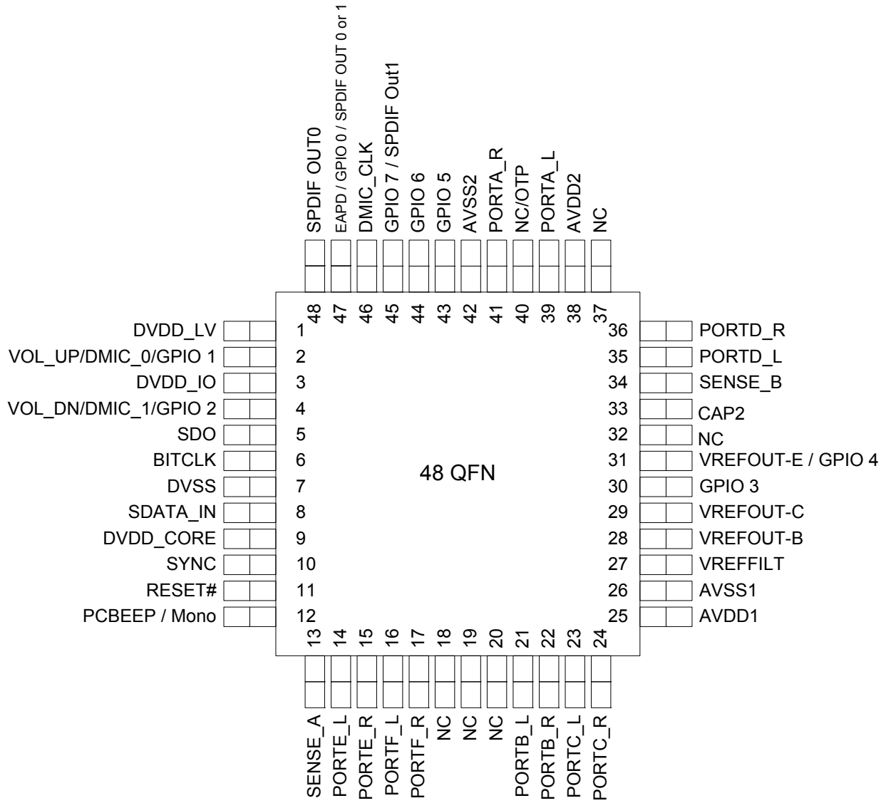
Figure 16. 48 Pad Assignment
