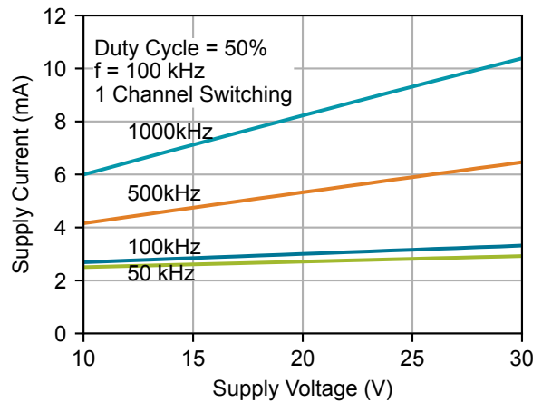
Figure 4.14. Supply Current vs. Supply Voltage ( C_L = 100 pF)
